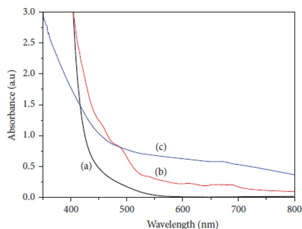
Figure 4. UV spectra of AMD (a), RBE (b), and iron nanoparticles (c); sample EK35.
