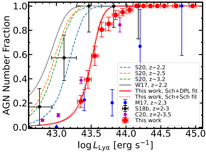
Figure 11. The AGN number fraction as a function of \log L_{\text{Ly}\alpha} . Our results derived with Equation (12) are shown with red circles. The functional form of our f_{\text{AGN,Ly}\alpha} derived with Equation (13) using model 1 (2) is presented by the red solid (dashed) line. The other symbols represent previous measurements whose references are listed in the legend. M17: Matthee et al. (2017); W17: Wold et al. (2017); S18: Sobral et al. (2018b); C20: Calhau et al. (2020).
