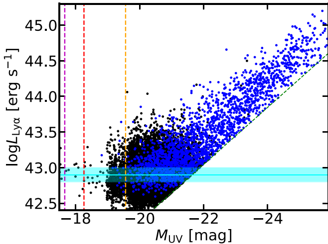
Figure 3. The M_{UV} - \log L_{Ly\alpha} distributions of our LAE sample. The blue (black) data points denote BL (NL) LAEs. The green dashed line indicates our EW_0 > 20 \text{ \AA} cut. The horizontal cyan line corresponds to our 50% L_{Ly\alpha} detection limit averaged over our redshift range, with the cyan shaded region indicating the 1\sigma uncertainty (68.27% equal-tailed credible interval). The magenta, red, and orange vertical dashed lines show the M_{UV} detection limits in the COSMOS, Fall, and Spring fields, respectively.
