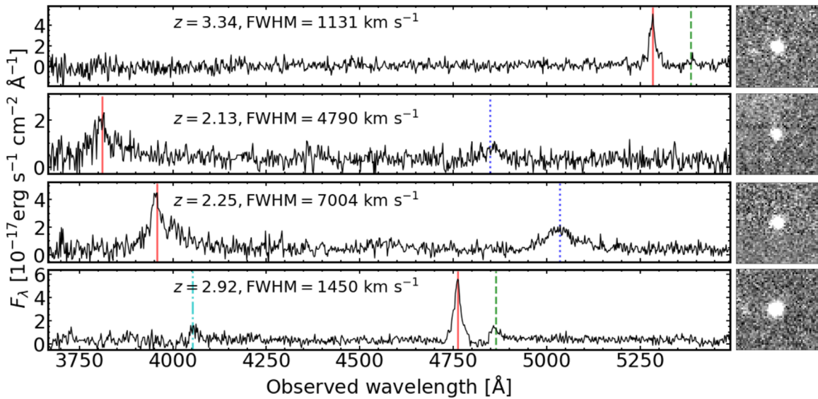
Figure 2. Same as Figure 1 but for our BL LAEs. Additionally, the blue dotted lines, green dashed lines, and cyan dashed-dotted lines represent the wavelengths of detected C IV, N V \lambda 1240 \text{ \AA} , and O VI \lambda 1035 \text{ \AA} emission lines, respectively.
