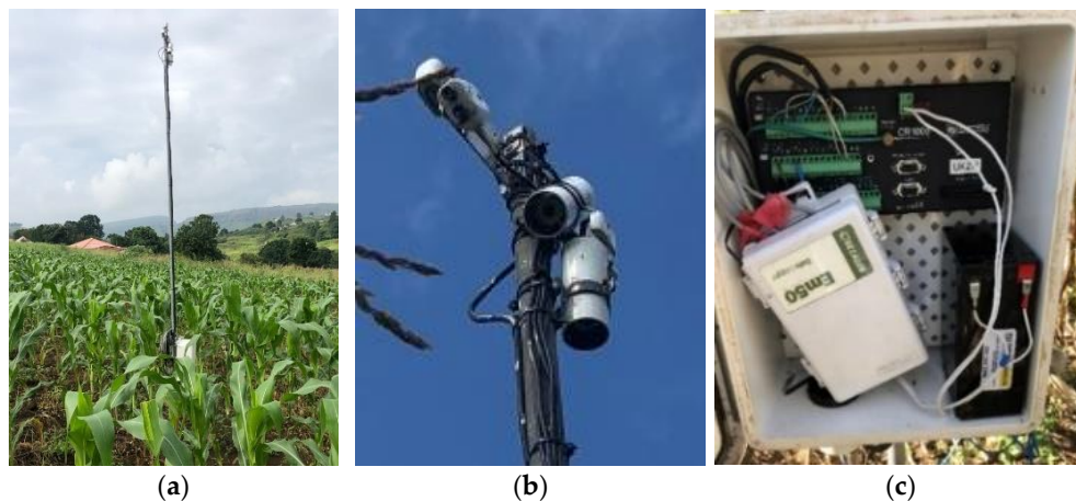
Figure 3. (a) Automated in-field meteorological tower in the maize field, (b) meteorological tower mounted with SI-111 Apogee IRR sensors held 4-m above the ground, (c) CR1000 data logger, Em50 data logger and 12 V battery.
