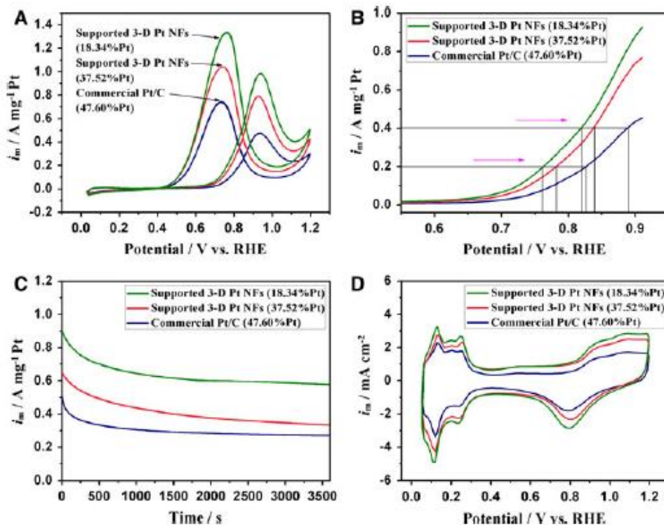
Fig. 2 a CV curves at 50 \text{ mV s}^{-1} . b Linear-sweep voltammograms. c Chronoamperometric curves at 0.90 V in an aqueous solution containing 0.5 M \text{H}_2\text{SO}_4 and 1 M methanol. d CV curves at 50 \text{ mV s}^{-1} in \text{N}_2 -sparged 0.5 M \text{H}_2\text{SO}_4 solution. All these curves were recorded at a temperature of 25^\circ\text{C}
