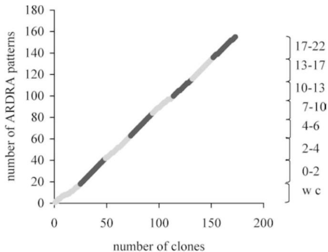
Fig. 1 Rarefaction curve for the different ARDRA patterns of 16S rDNA clones. Between 25 and 30 clones from each library [library from water column ( wc ), 0-2 cm, 2-4 cm, 4-6 cm, 7-10 cm, 10-13 cm, 13-17 cm, and 17-22 cm of sediment depth] were analyzed
