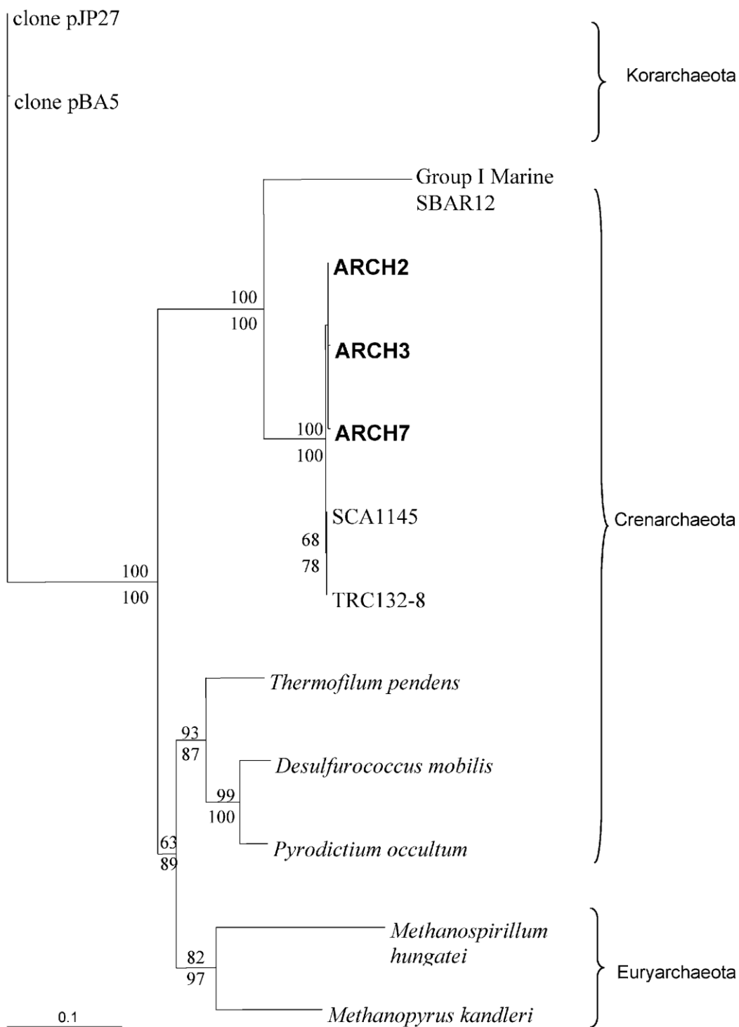
Fig 3 Phylogenetic tree of archaeal 16S rDNA clones derived from Bratina Island pond sediment 10-13 Cm. Names in bold are representative clones of the detected phylotypes with selected reference sequences. The bar represents 10% estimated sequence divergence
