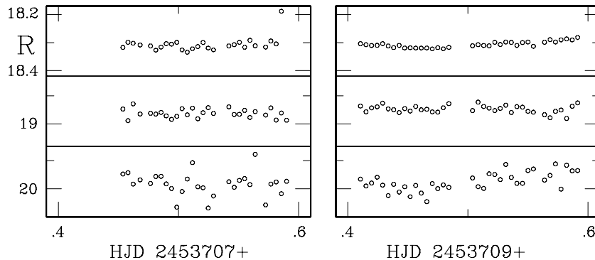
Figure 2. R_C -band observations of 2M 0605–22342 (bottom panels) and two other stars in the field of view. The vertical scale on all axes is 0.25 mag.
