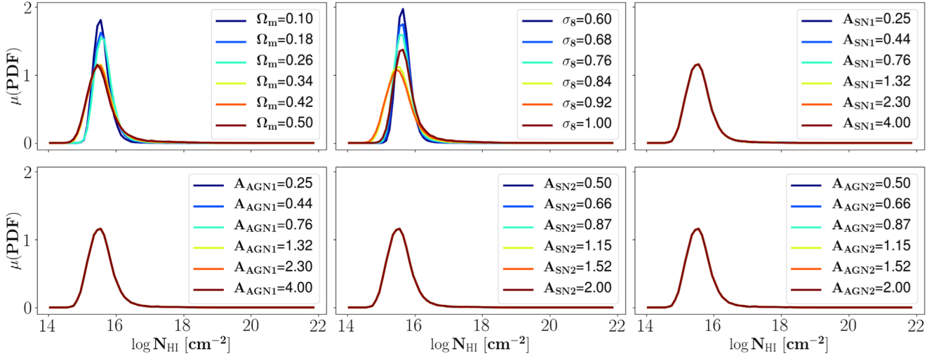
Figure 4. Impact of varying a single CAMELS parameter on the mean pdf over 15 HI maps, sharing the same parameters using the IP set. As is evidenced by the amount of variation in the mean pdf ( \mu(\text{pdf}) ), the HI maps are mostly affected only by the cosmological parameters ( \Omega_m and \sigma_8 ) and not the astrophysical parameters ( A_{\text{SN}1} , A_{\text{SN}2} , A_{\text{AGN}1} , and A_{\text{AGN}2} ); hence we choose to condition HIFLOW solely on cosmology.
