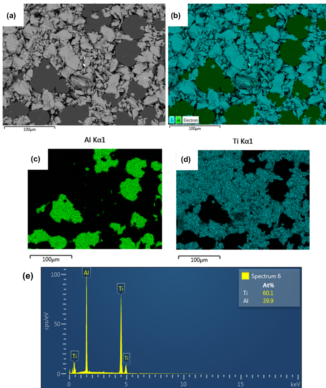
Fig. 4. SEM-EDS elemental map analysis for the Ti-48Al alloy: (a) electron image, (b) EDS layered image, (c) Al K \alpha , (d) Ti K \alpha , and (e) spectra with corresponding atomic composition.
