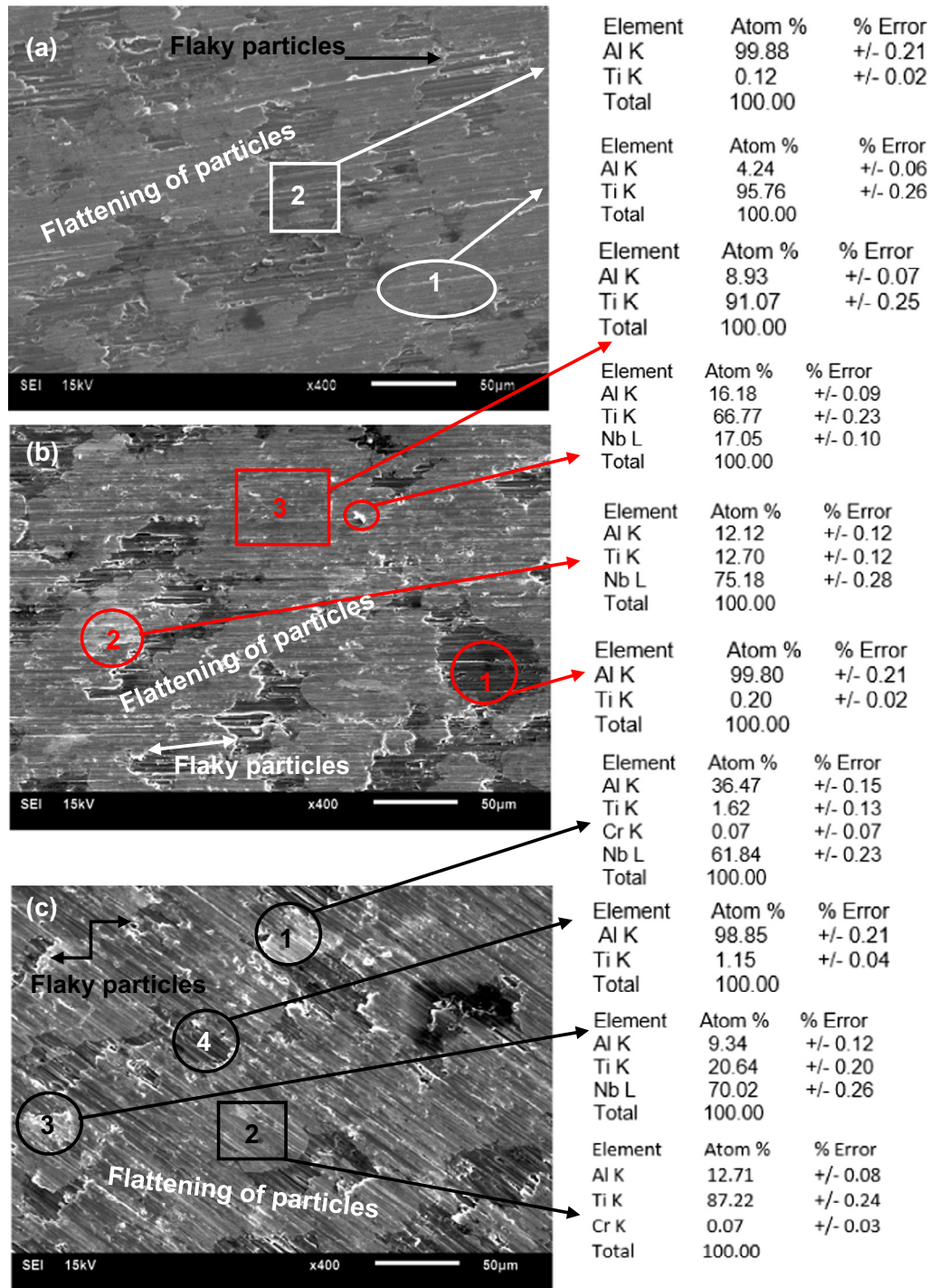
Fig. 7. SEM/SEI micrographs of (a) Binary Ti-48Al. (b) Ternary Ti-48Al-2Nb and (c) Quaternary Ti-48Al-2Nb-0.7Cr compacted alloy powders, further away from the surface.
