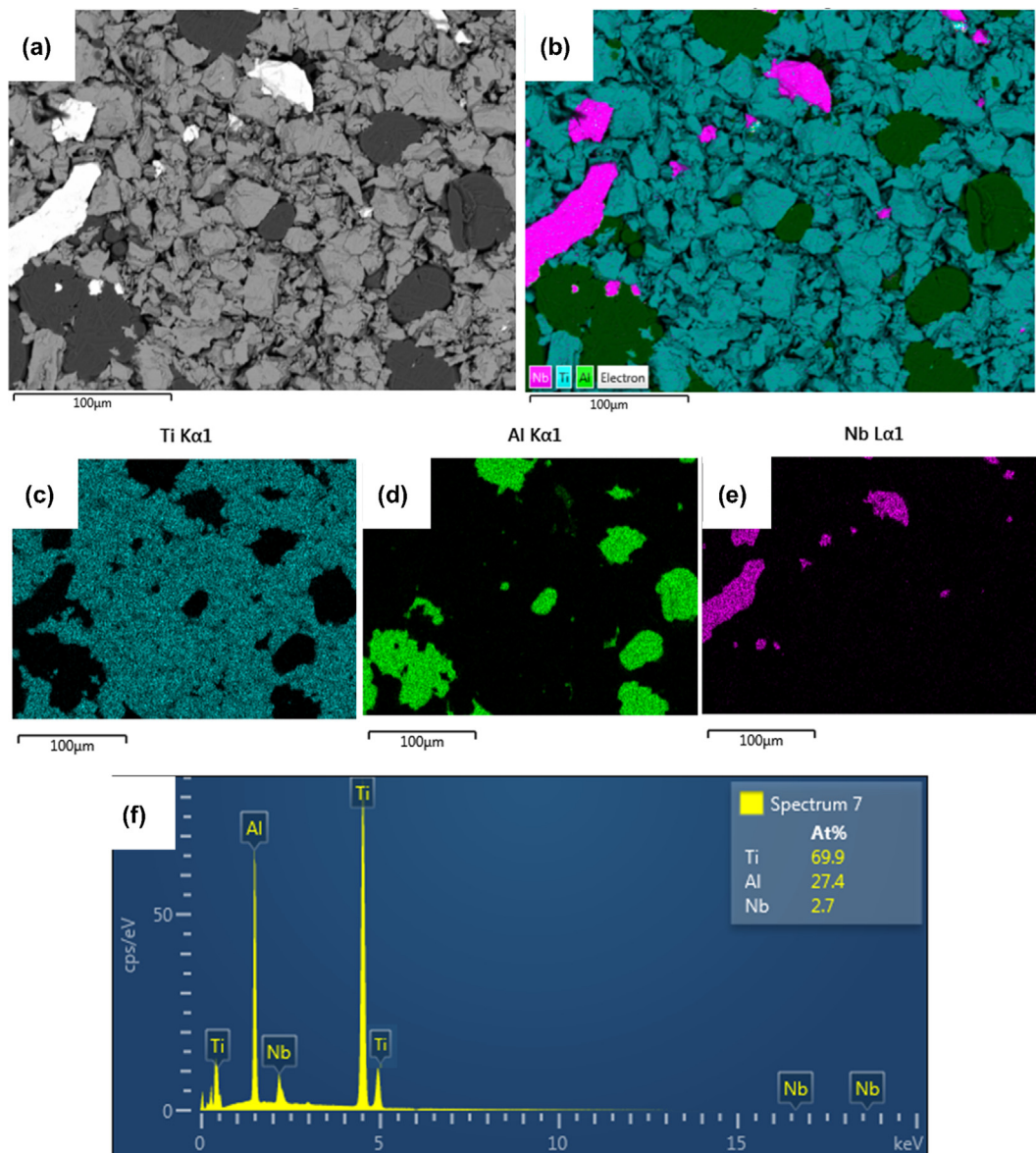
Fig. 5. SEM-EDS elemental map analysis for the Ti-48Al-2Nb alloy: (a) electron image, (b) EDS layered image, (c) Ti K\alpha , (d) Al K\alpha (e) Nb L\alpha , and (f) spectra with corresponding atomic composition.
