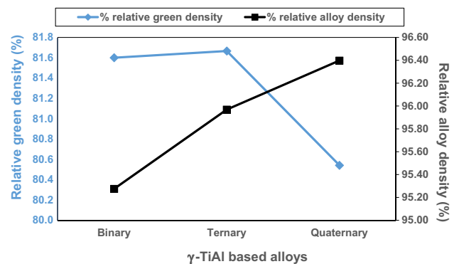
Fig. 13. Comparative relative densities between the green compacts and the arc melted buttons. (For interpretation of the references to colour in this figure legend, the reader is referred to the web version of this article.)
