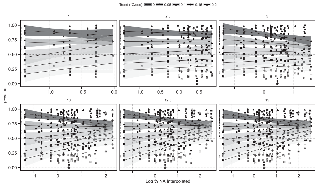
FIG. 7. The relationship between the amount of missing values (log % NA) and the significance of a modeled trend ( p value). Each panel shows the effect of an increasingly larger amount of missing values indicated above each panel by numerals (from top left to bottom right): 1, 2.5, 5, 10, 12.5, and 15. The fitted black lines and 95% confidence intervals (shown as gray-shaded bands) represent each of the five decadal trends assessed ( ^{\circ}\text{C decade}^{-1} ) shown using different black symbols: 0 (circles), 0.05 (triangles), 0.1 (squares), 0.15 (crosses), and 0.2 (squares with an \times symbol inside).
