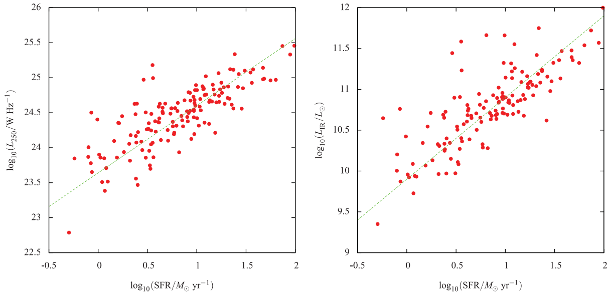
Figure 9. The relationship between SFR, determined for the SF class from the MPA-JHU emission-line data base using the methods of Brinchmann et al. (2004), and the two types of FIR luminosity discussed in this paper, L_{250} (left) and L_{\text{IR}} (right). The green lines show the results of a MCMC regression, as described in the text. Error bars are not plotted for clarity – the uncertainty on SFR can be \pm 0.5 dex.
