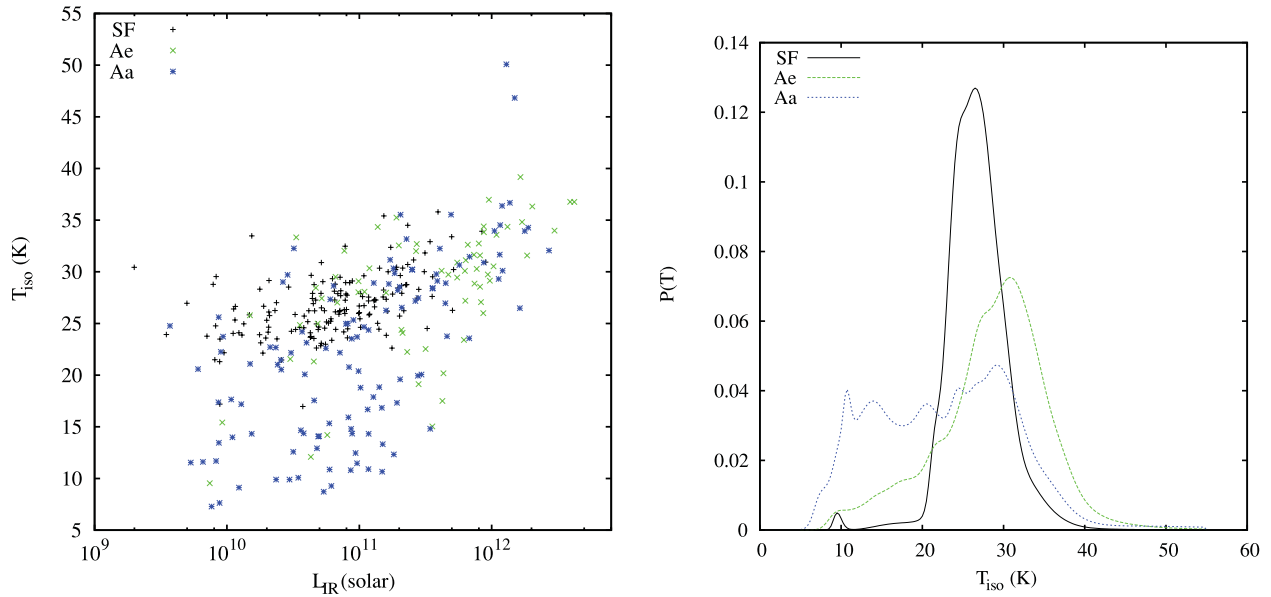
Figure 7. Left: a temperature–luminosity plot for the SF, Aa and Ae sources with individually determined temperatures. Right: stacked, normalized PDFs for temperature fits to the SF, Ae and Aa emission-line classes.
