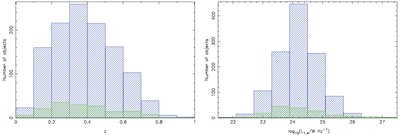
Figure 3. The distribution of (left) redshift and (right) radio luminosity in the Aa (blue) and Ae (green) objects after the SF cut. The redshift and luminosity distributions of the samples are very similar.
