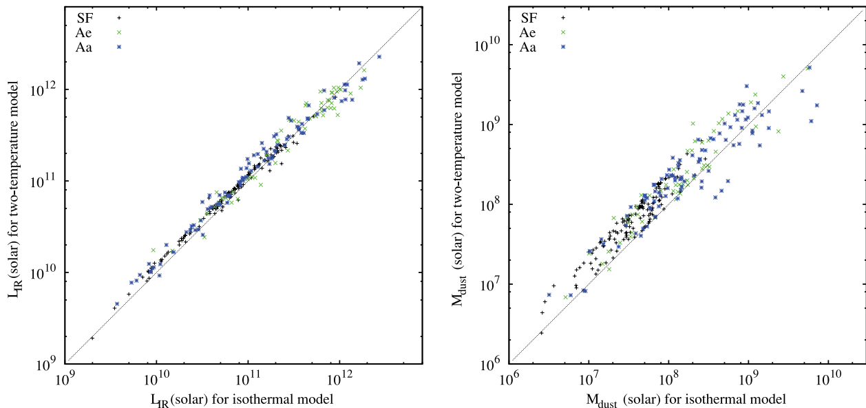
Figure 8. The relationships between (left) the integrated IR luminosity and (right) the dust mass for objects with fits of both a single-temperature and a two-temperature model.
