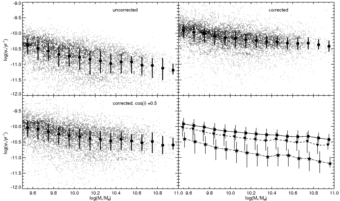
FIG. 5.— Specific star formation rate \psi_* as a function of stellar mass M_* for a subsample of the OPTICAL sample with 7.6 \leq \log(\mu_*) \leq 9.0 and M_* > 10^{9.5} M_\odot . The relation is shown before correction for attenuation by dust (top left panel), after the full inclination-dependent correction, described in § 5.1, using the PT11 model in conjunction with the \tau_B^f - \mu_* relation (top right panel), and after a partial correction using the procedure of § 5.1 but artificially setting a uniform inclination i_d with \cos(i_d) = 0.5 for all galaxies (lower left panel). The sources are binned in 15 bins of equal size in M_* , with the median depicted by a filled circle, and the bars showing the interquartile range. The scatter in the relation due to the scatter in the NUV is reduced from the uncorrected to the fully corrected case. The intrinsic values of \psi_* are shifted upwards w.r.t. the uncorrected values. The linear gray-scale shows the number density of sources at that position, with the same scale having been applied to all samples. The median values and interquartile ranges are shown together in the bottom right panel. The uncorrected values are depicted by stars and a dash-dotted line, the values corrected at a fixed inclination of \cos(i) = 0.5 are shown as inverted triangles and a dashed line, and the fully corrected values are shown as circles and a solid line. The bin centers have been offset by 0.01 in \log(M_*) for improved legibility.
