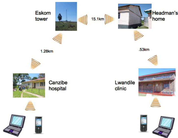
Figure 2. Canzibe/Lwandile network diagram
