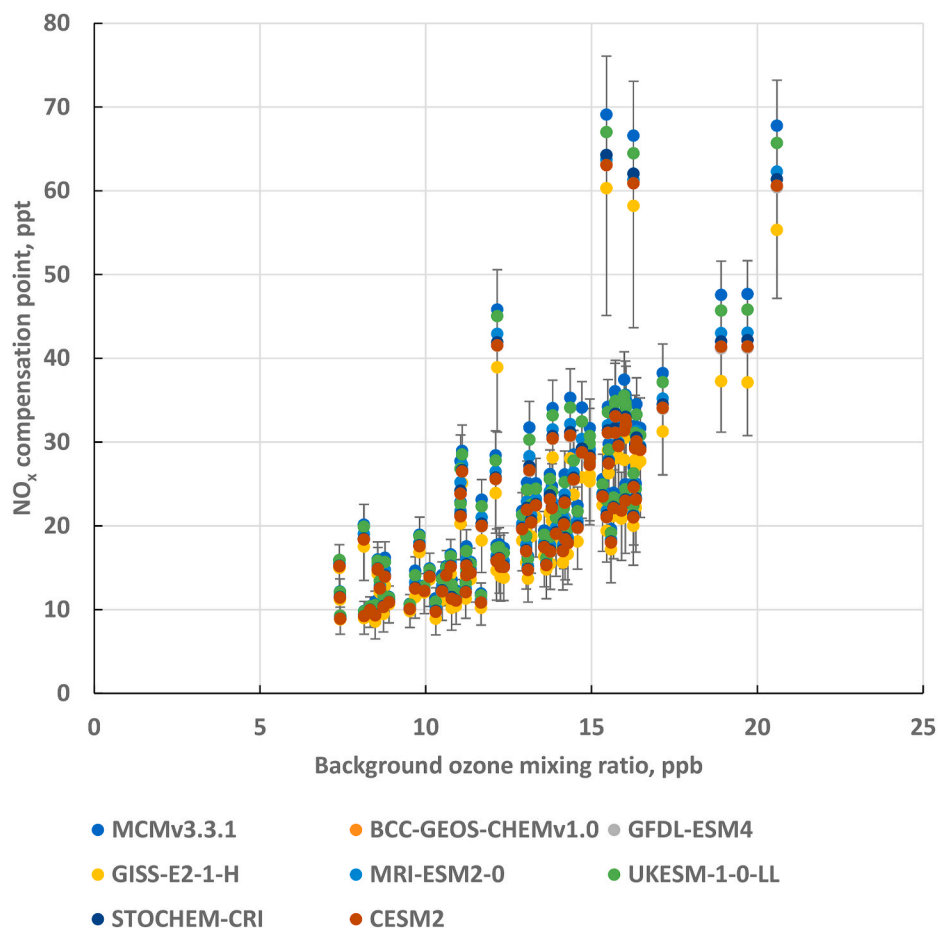
Fig. 1. Scatter plot of the \text{NO}_x compensation points determined at each background location versus the background ozone mixing ratio for each model chemical mechanism. The error bars shown are for CESM2-WACCM based on the maximum and minimum values found in the Monte Carlo uncertainty analysis.
