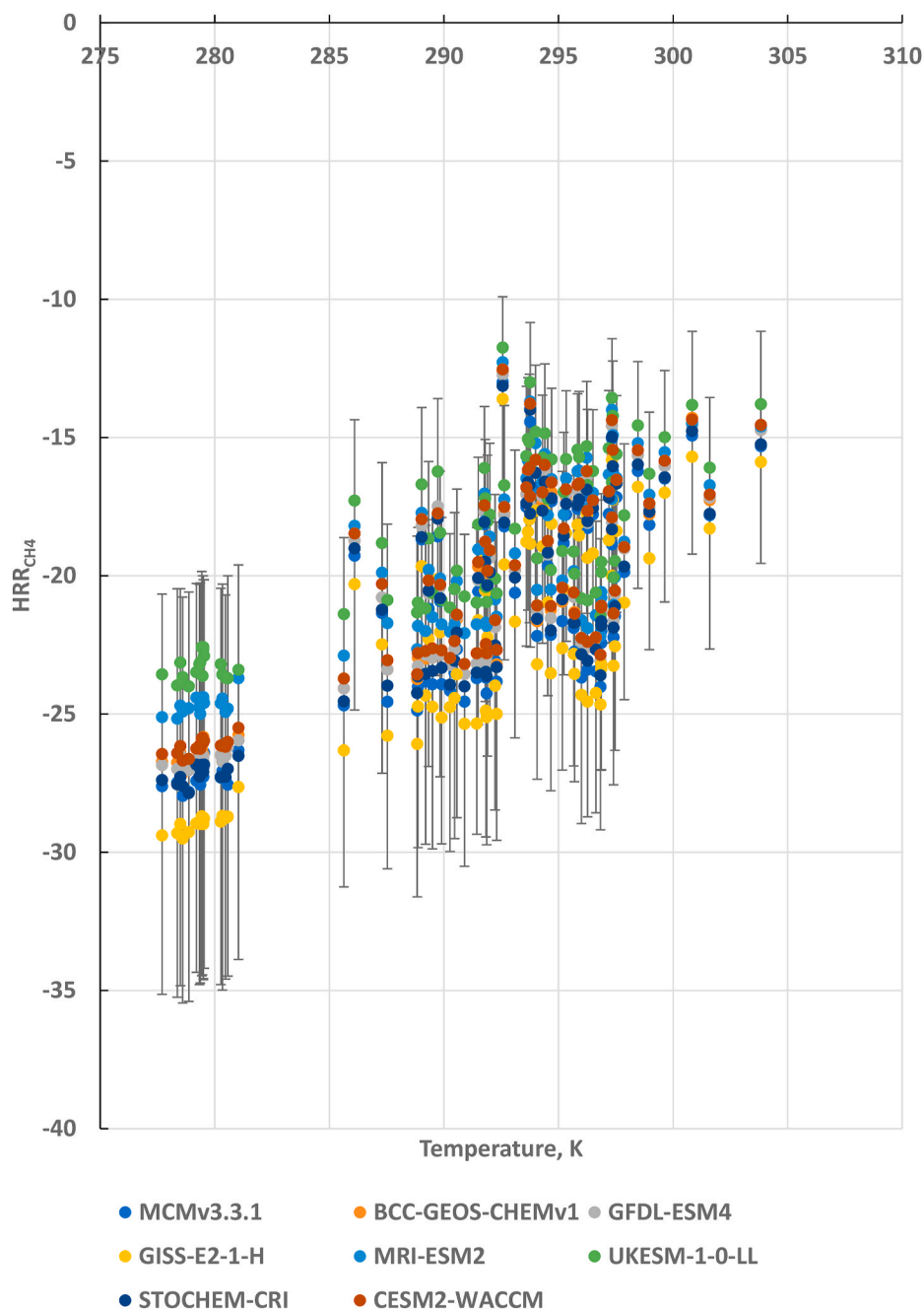
Fig. 2. Scatter plot of the HRR_{CH_4} values determined at each background location versus the background temperature for each model chemical mechanism. The error bars shown are for CESM2-WACCM based on the maximum and minimum values found in the Monte Carlo uncertainty analysis.
