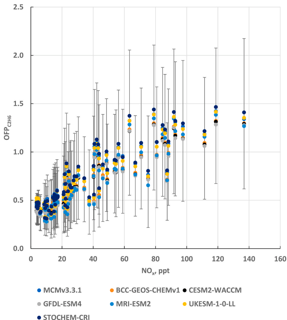
Fig. 4. Scatter plot of the OFP_{C_2H_6} values versus the background NO_x at each background location for each model chemical mechanism. The error bars shown are for CESM2-WACCM based on the maximum and minimum values found in the Monte Carlo uncertainty analysis.
