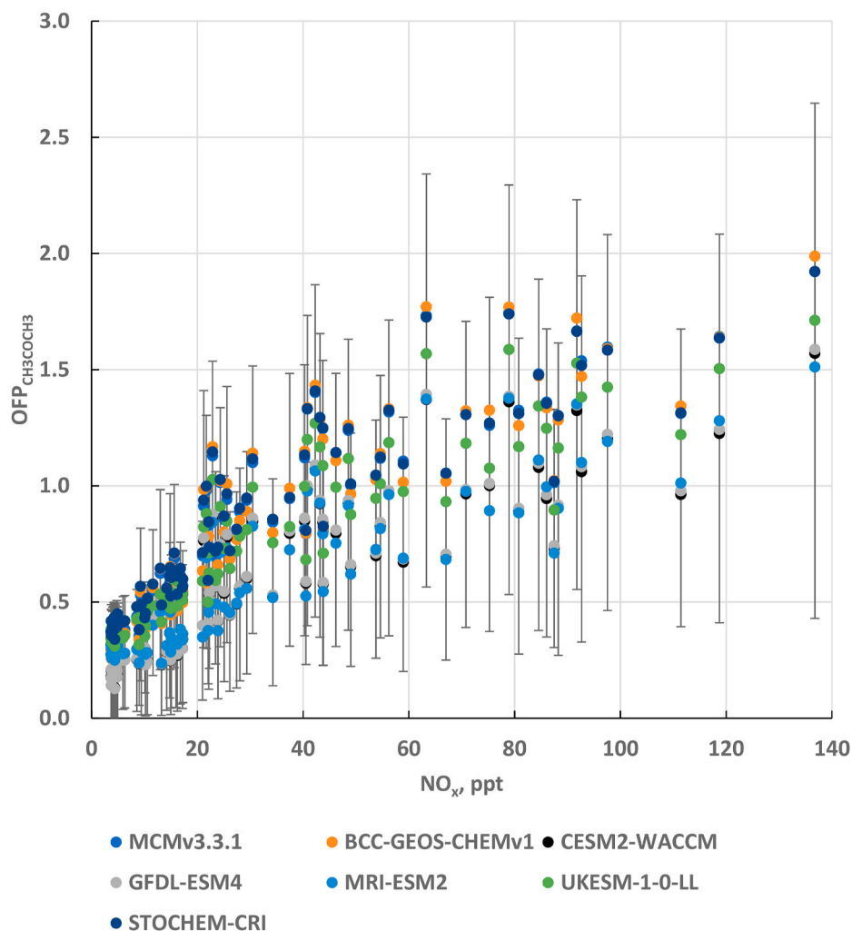
Fig. 6. Scatter plot of the OFP_{CH_3COCH_3} values versus the background NO_x at each background location for each model chemical mechanism. The error bars shown are for CESM2-WACCM based on the maximum and minimum values found in the Monte Carlo uncertainty analysis.
