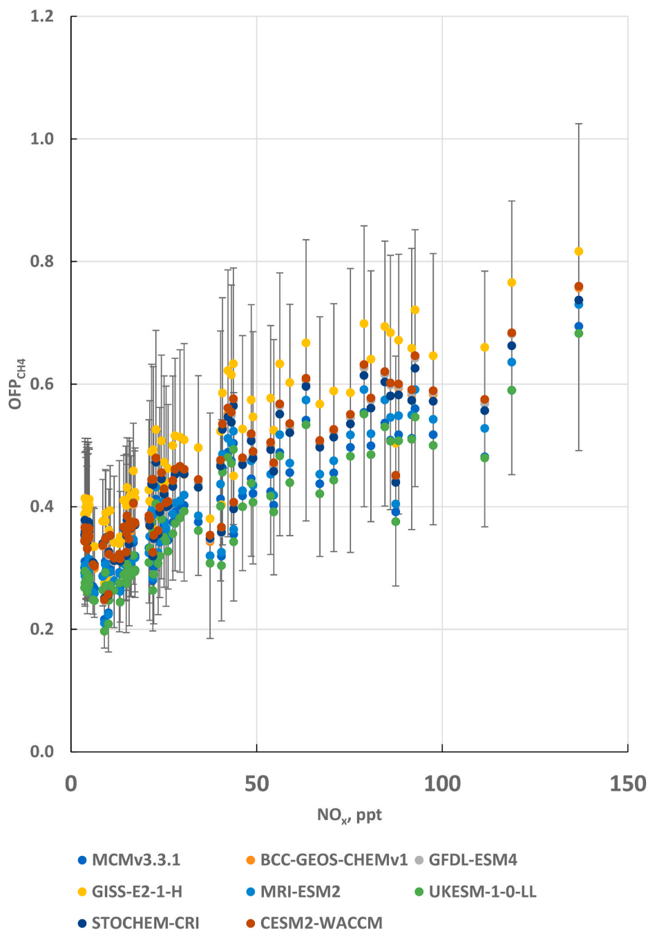
Fig. 3. Scatter plot of the \text{OFP}_{\text{CH}_4} values versus the background \text{NO}_x at each background location for each model chemical mechanism. The error bars shown are for CESM2-WACCM based on the maximum and minimum values found in the Monte Carlo uncertainty analysis.
