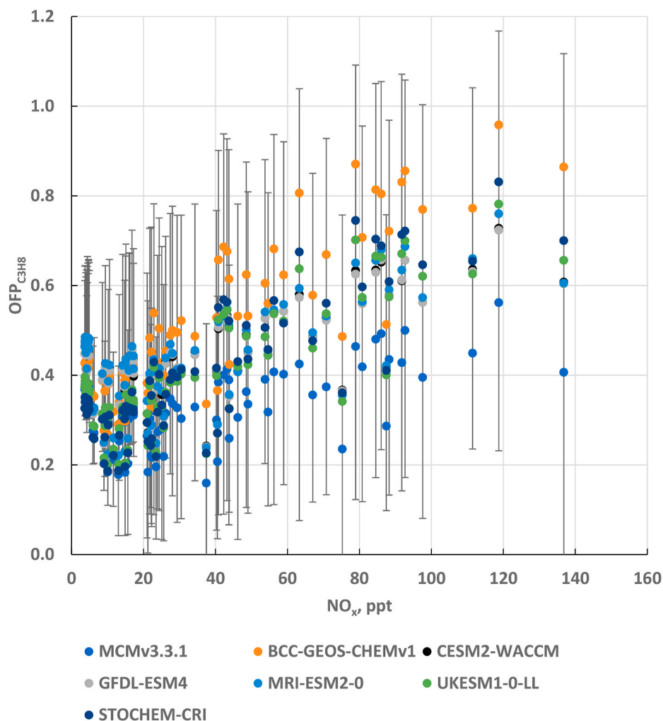
Fig. 5. Scatter plot of the OFP_{C_3H_8} values versus the background NO_x at each background location for each model chemical mechanism. The error bars shown are for CESM2-WACCM based on the maximum and minimum values found in the Monte Carlo uncertainty analysis.
