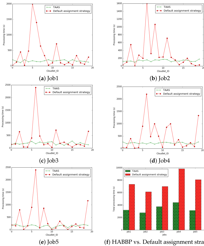
Figure 10. Processing time of the cloudlets in Job 1, Job 2, Job 3, Job 4 and Job 5.
