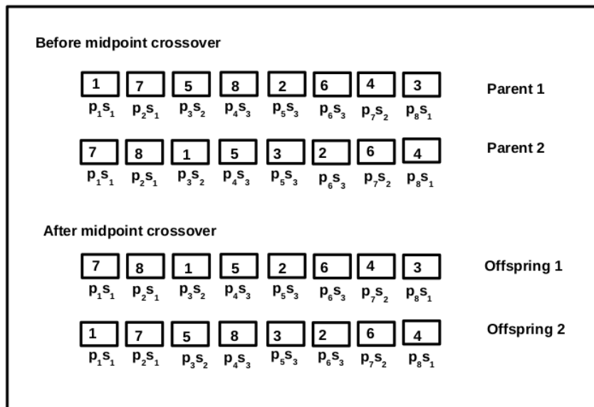
Figure 4. Midpoint crossover.
