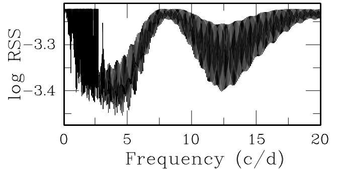
Figure 4. A residual sum-of-squares periodogram (see text) of the observations of DENIS 0255–4700.
