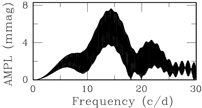
Figure 2. Amplitude spectrum of the detrended, combined I_C band observations of DENIS 0255–4700.
