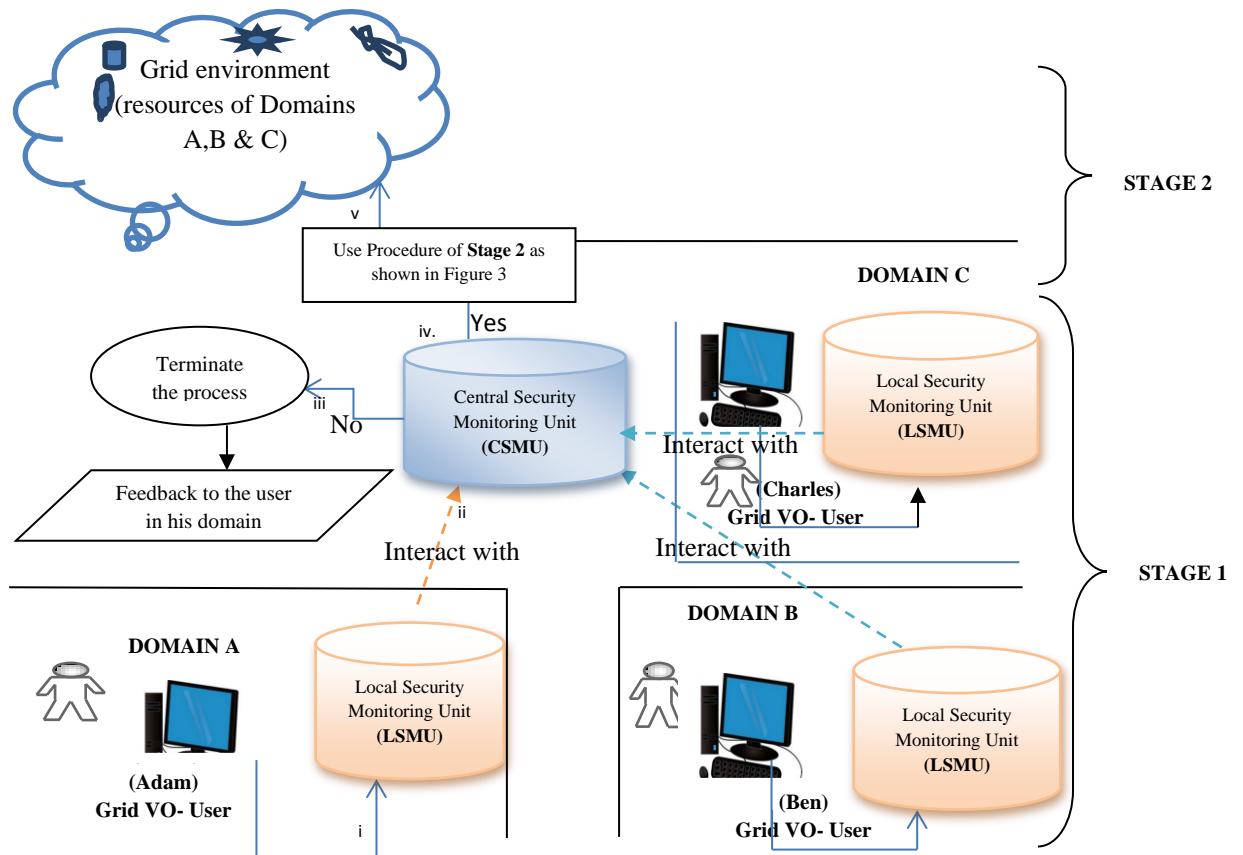
Figure 2. A 3-domain role based access control architecture showing interaction between users, CSMU and LSMU
