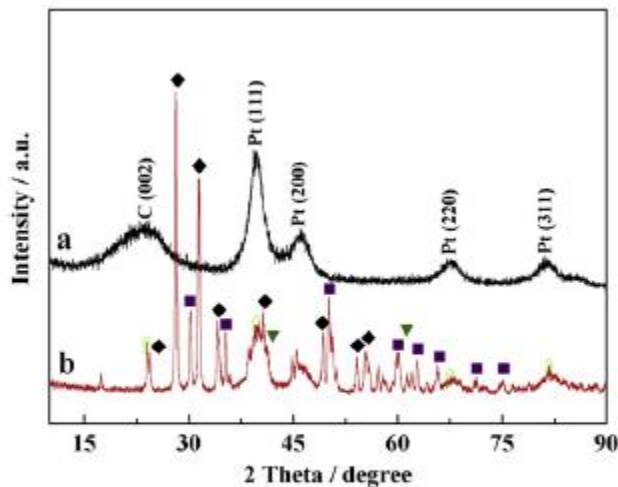
Fig. 2 – XRD patterns of (a) Pt/C@CN_x and (b) Pt/ZrO_2@CN_x , ( \blacklozenge ) ZrO_2 monoclinic, ( \blacksquare ) ZrO_2 tetragonal, ( \blacktriangledown ) ZrO_2 cubic).
