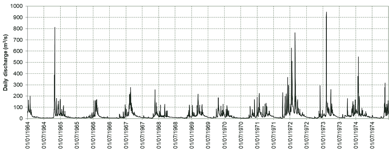
Figure 2 Daily pre-Jozini Dam discharge of the Pongola River at Gauge W4H013 (1965–1974)
