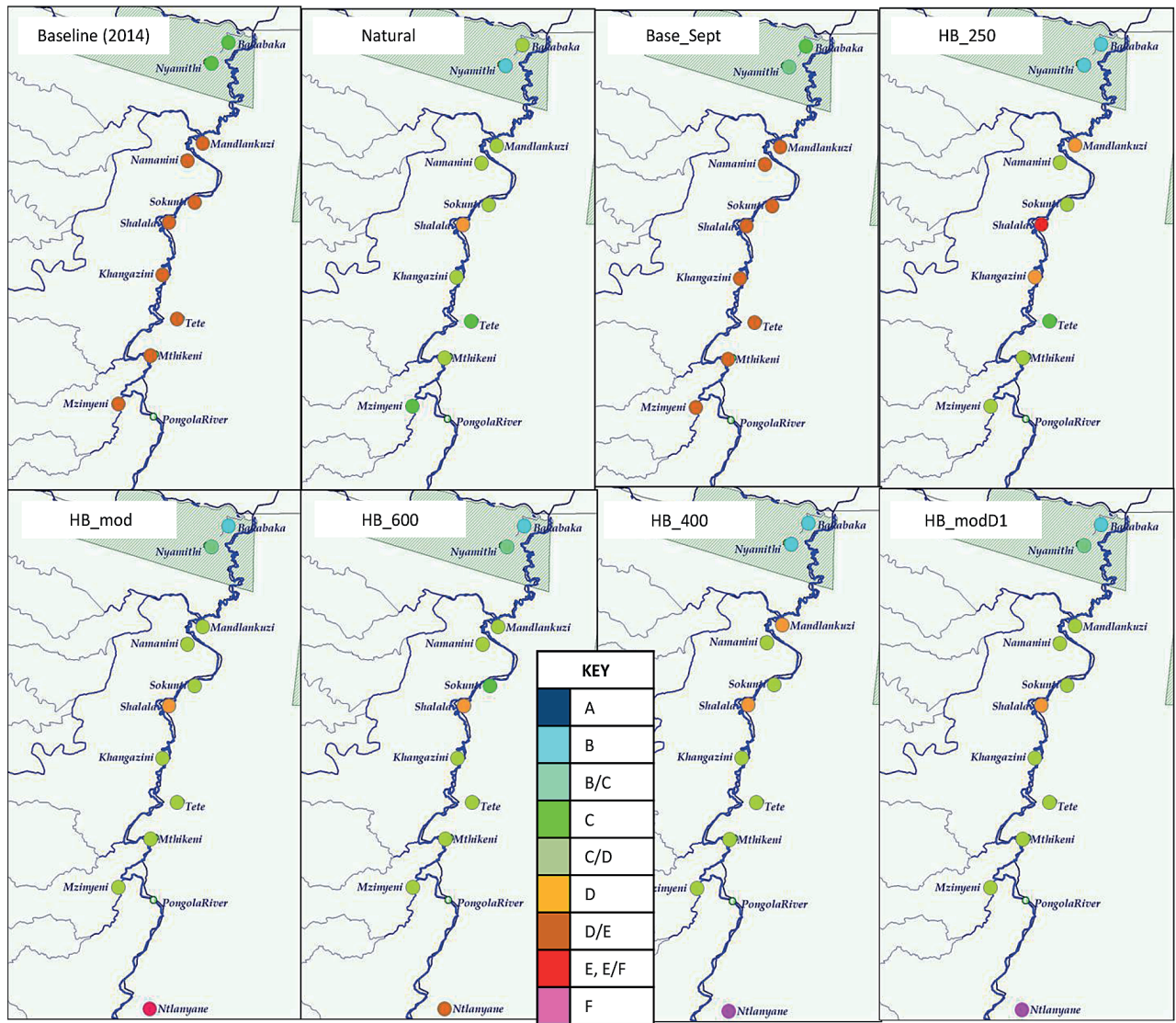
Figure 8 Estimated ecological condition for the study sites under each of the scenarios
