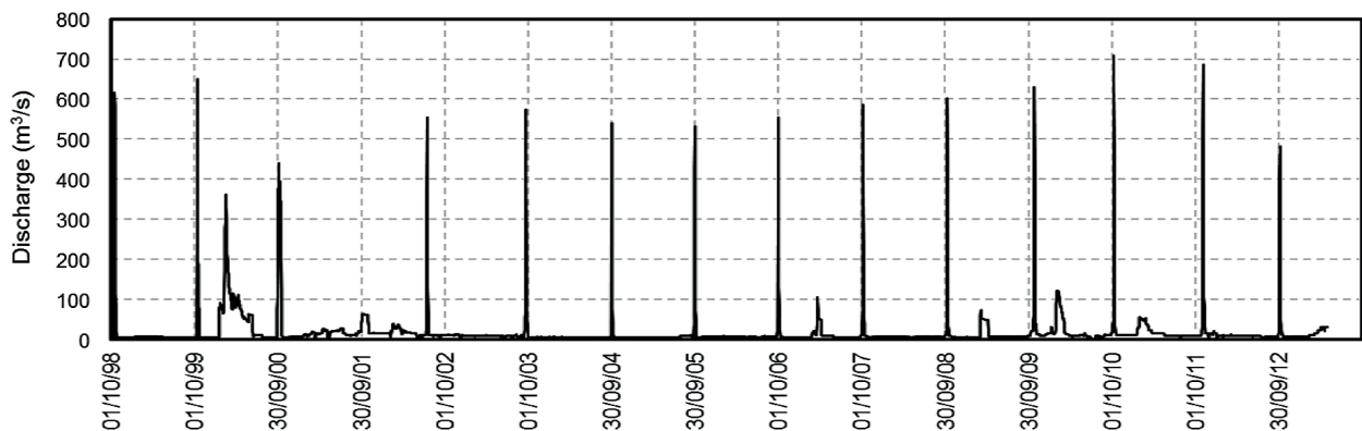
Figure 3 Releases from Jozini Dam into the Pongola River gauged at Station W4H013 (1998 to 2012)
