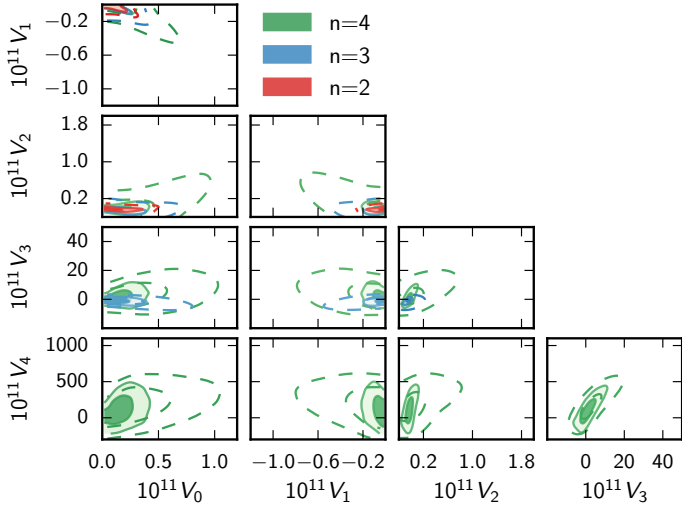
Fig. 11. Taylor expansion of V(\phi) at order n = 2, 3, and 4 in the observable region, making no assumption about the end of inflation. In natural units (where \sqrt{8\pi M_{\text{Pl}}} = 1 ). The parameters are the Taylor coefficients, obtained here as derived parameters with non-flat priors. Dashed contours are Planck TT,TE,EE+lowE, while solid contours are Planck TT,TE,EE+lowE+lensing+BK15. The scales are the same as in PCI15.
