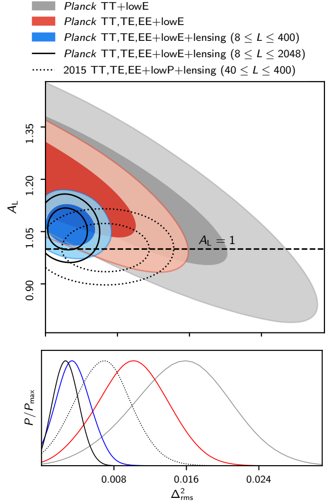
Fig. 47. Degeneracy between A_L and \Delta_{\text{rms}}^2 in the \Lambda CDM+ A_L +CIP model (top panel) and constraints on \Delta_{\text{rms}}^2 in the \Lambda CDM+CIP model, where A_L = 1 (bottom panel).
