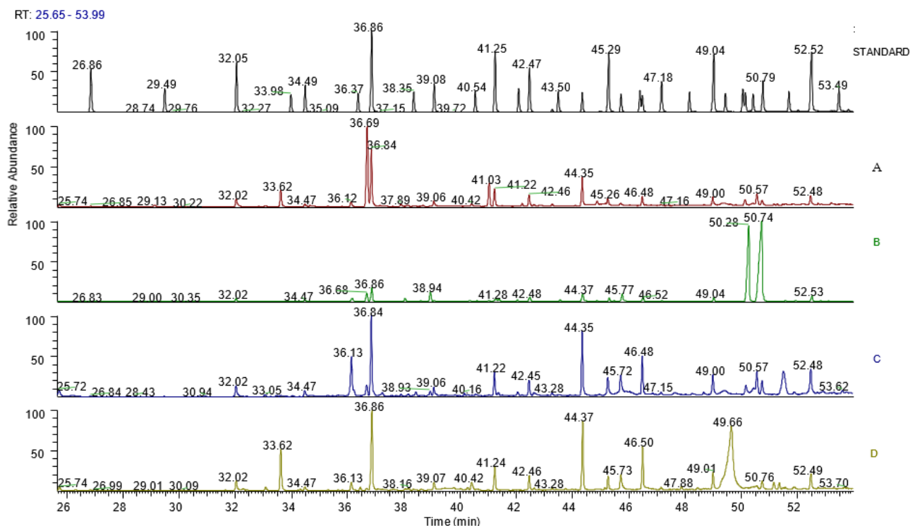
Figure 5. Shows the GC-MS chromatogram of the fatty acids of aqueous acetone extract of H. pandurifolium , H. foetidum , H. petiolare , and H. cymocum with regularly labelled signals detected by the GC-MS detector. LEGEND: (A)—FAMES chromatogram of H. pandurifolium ; (B)—FAMES chromatogram of H. foetidum ; (C)—FAMES chromatogram of H. petiolare ; (D)—FAMES chromatogram of H. cymocum .
