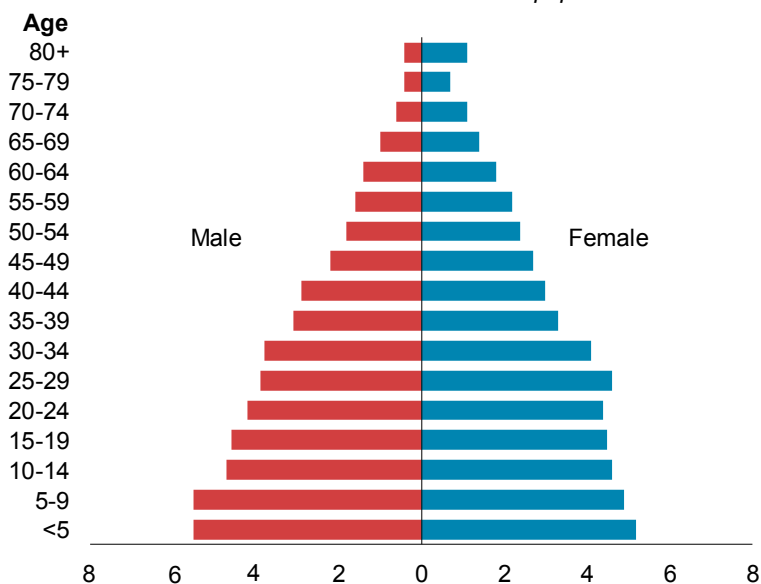
Figure 2.5 Population pyramid
