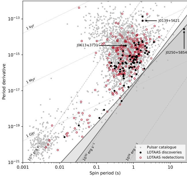
Fig. 8. P – \dot{P} diagram of the pulsars discovered (black dots) and red-detected (red circles) by the LOTAAS survey and the known pulsar population (grey dots). The grey dotted and dashed diagonals represent the characteristic ages and the spin-down luminosities, respectively. The solid lines are deathlines from Chen & Ruderman (1993) and Zhang et al. (2000) .
