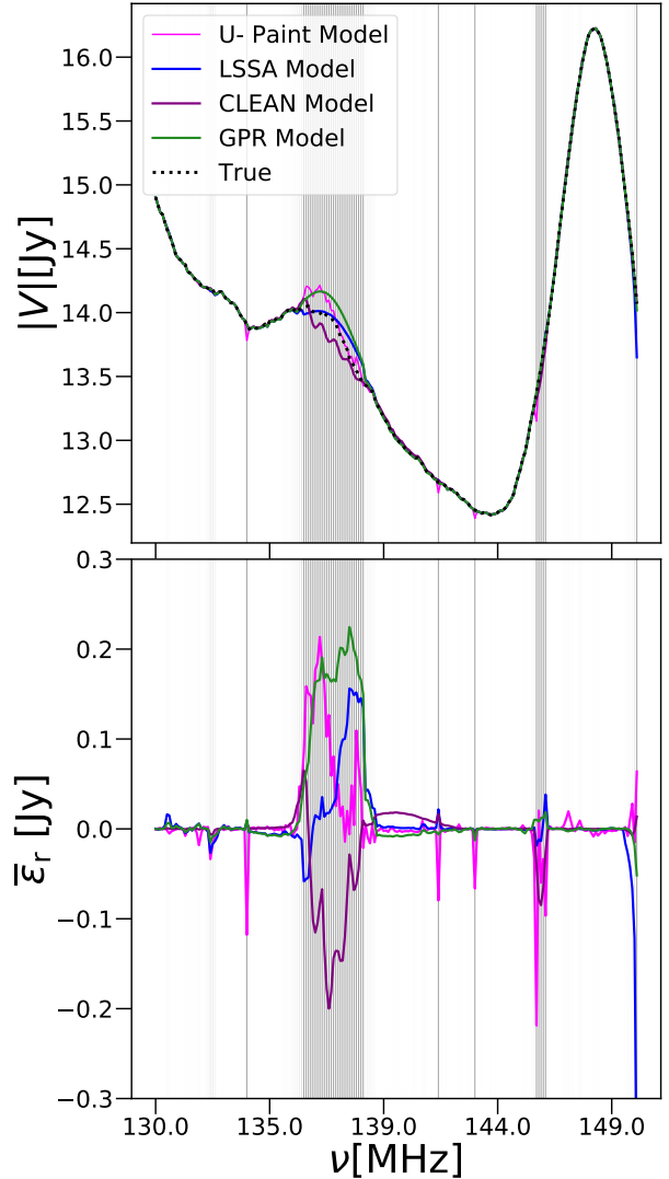
Figure 5. Top: LST averaged inpaint model visibilities. The true visibilities are shown with the dotted black curve. The vertical shaded regions correspond to the RFI flagged channels. The amount of shade is proportional to the frequency in which those channels are flagged. Thus the Wideband OR-BCOMM feature is darkest since it is always flagged. Note that the inpaint models are only filled into RFI gaps, and so the inpaint models only deviate from the true visibilities in shaded regions. The orange curve corresponds to U-Paint, the yellow curve to LSSA, purple curve to CLEAN and blue curve to GPR. DPSS models are not shown since we feature the wideband feature in this image (see Section 3). Bottom: The residuals between inpaint models and the true visibilities.
