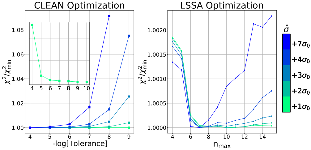
Figure 2. The results of our parameter optimization procedure for CLEAN and LSSA inpainting methods. In the left image fractional increase in \chi^2 is plotted as a function of tolerance parameter values (see Section 3.1). The coloured curves represent different noise levels. As the thermal noise level in the dataset increases the optimal tolerance decreases. The inset provides a closer examination of \chi^2/\chi_{\min}^2 for fiducial noise level \alpha = 1 . Similarly on the right image, the fractional increase in \chi^2 is plotted as a function of n_{\max} , the number of Fourier components to include in LSSA models. As we increase the thermal noise of the dataset, the optimal number of Fourier components to include in the model decreases.
