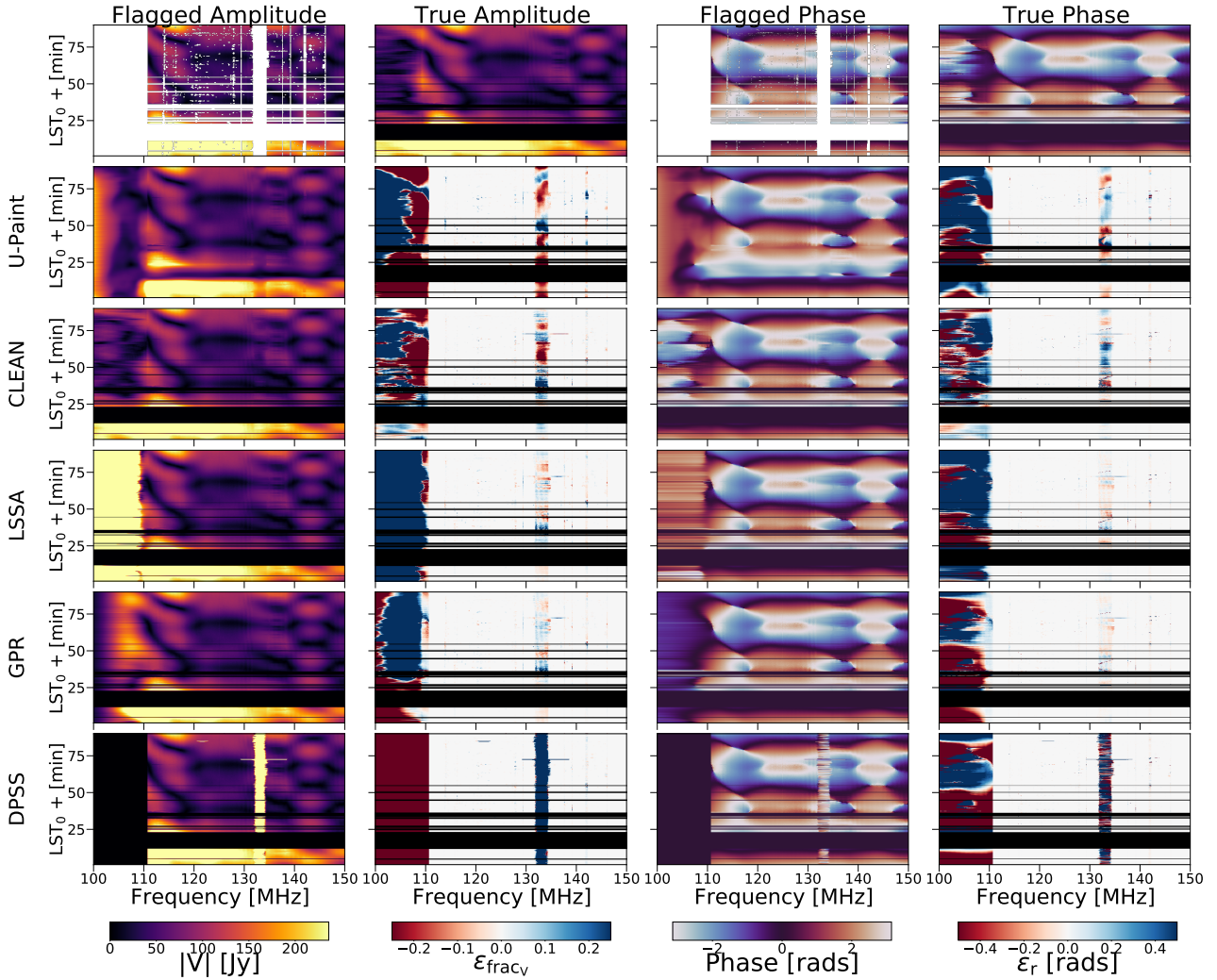
Figure 12. Same as Figure 4 but with the PIV visibilities from Section 2.3. The true visibilities in the first row (second and fourth column) have been initially inpainted with the CLEAN algorithm to generate placeholder data for the RFI flagged regions. The inpaint techniques are then applied to a set of flags which are shifted 40 channels to the left. This is done in order to avoid inpainting over the already CLEANed data. See Section 8 for more details regarding our procedure. Note that as compared to Figure 4 the fractional errors in the model visibilities increase.
