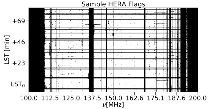
Figure 1. Sample HERA flags split from 100MHz-200MHz. Frequency channels below 110MHz are reserved for FM radio. The ORBCOMM satellite is responsible for RFI at \nu = 136\text{MHz} . Frequency channels above \nu = 174\text{MHz} are flagged due to broadcast television.
