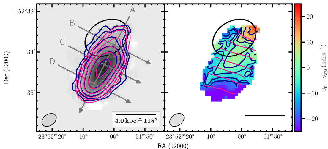
Figure 3. MeerKAT H I total-intensity map and moment-1 velocity field, as derived from the data cube shown in Figs 2, A1, and A2. Blue: derived from the observation. Pink: derived from the TiRiFiC model. The white cross or the intersection between arrows A and C represents the kinematical centre of the model, the ellipse to the lower left the synthesised beam ( HPWB ), the black ellipse to the top highlights the position of kinematically anomalous gas. Left-hand panel: total-intensity map. Contours denote the 0.25, 0.5, 1, 2, 4, 8- M_{\odot} \text{pc}^{-2} -levels. Arrows indicate the positions of slices along which the position-velocity diagrams in Fig. 7 were taken. Right-hand panels: velocity field. Contours are isovelocity contours. They denote the -15, -10, -5, 0, 5, 10, 15 \text{ km s}^{-1} -levels relative to the systemic velocity v_{\text{sys}} = 578 \text{ km s}^{-1} . A version showing only the data derived from the observed data cube can be found in the appendix (Figs A3).
