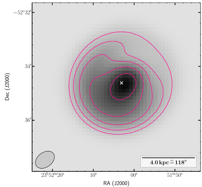
Figure A5. Face-on total-intensity map of the TiRiFiC model. The H I disc is simulated to be seen face-on, but at the same distance and the same resolution as compared to the observations. Contours: 0.25, 0.5, 1, 2, and 4 M_{\odot} \text{pc}^{-2} .
