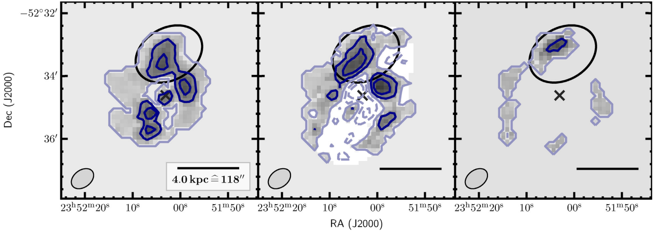
Figure 8. Difference total-intensity maps as derived shows that an initial increase of the dispersd from TiRiFiC model and observed data cube. Contours denote the -0.5, -0.25, 0., 0.25, 0.5 - M_{\odot} \text{pc}^{-2} -levels. Dashed contours show negative column-density levels, light blue corresponds to 0 M_{\odot} \text{pc}^{-2} . Left-hand panel: moment-0 derived from the difference data cube (observed - model). Middle panel: difference of the moment-0 of observation and model as shown in the left-hand panel of Fig. 3. Right-hand panel: Moment-0 taken from the data cube applying mask as used for deriving the moment-0 shown in the left-hand panel of Fig. 3 and additionally masking out the model data cube.
