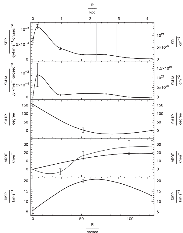
Figure 6. Final TiRiFiC model of the H I disc of ESO 149-G003. SBR/SD: surface brightness or surface column density. The two lines denote r_{25} and r_{\text{HI}} (at the larger radius). SM1A: amplitude of a harmonic distortion in surface brightness/surface column density. SM1P: phase of a harmonic distortion in surface brightness/surface column density. VROT: rotation velocity. The grey line is the result of a fit, in which the RC was left to vary on the nodes shown as dots. DISP: dispersion.
