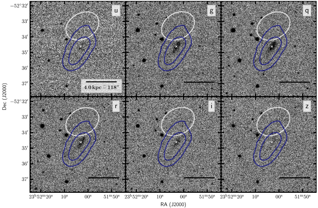
Figure A6. MeerLICHT observations of ESO 149-G003. Contours denote the 1, 4- M_{\odot} \text{ pc}^{-2} -levels of the observed total-intensity map shown in Figs 3 and A3. The white ellipse at the top highlights the position of kinematically anomalous H I.
