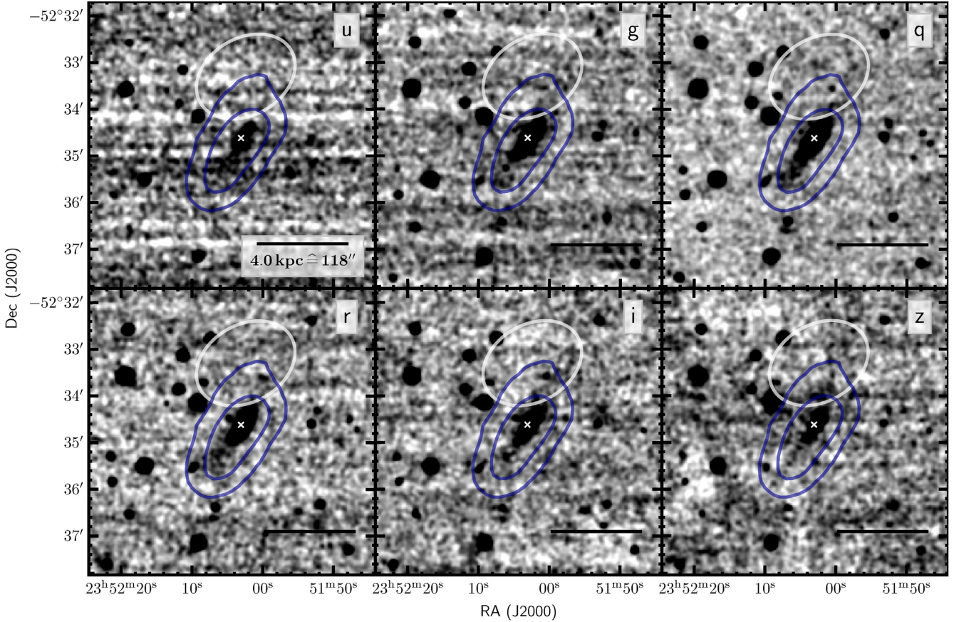
Figure 4. MeerLICHT observations of ESO 149-G003, convolved with a 2D-Gaussian of FWHM = 6 arcsec in each direction (RA and Dec.). Contours denote the 1, 4 - M_{\odot} \text{ pc}^{-2} -levels of the observed total-intensity map shown in the left-hand panel of Figs 3 and A3. The white ellipse to the top highlights kinematically anomalous gas. The white cross represents the kinematical centre of the kinematical model. The full-resolution maps can be found in Fig. A6 in the appendix.
