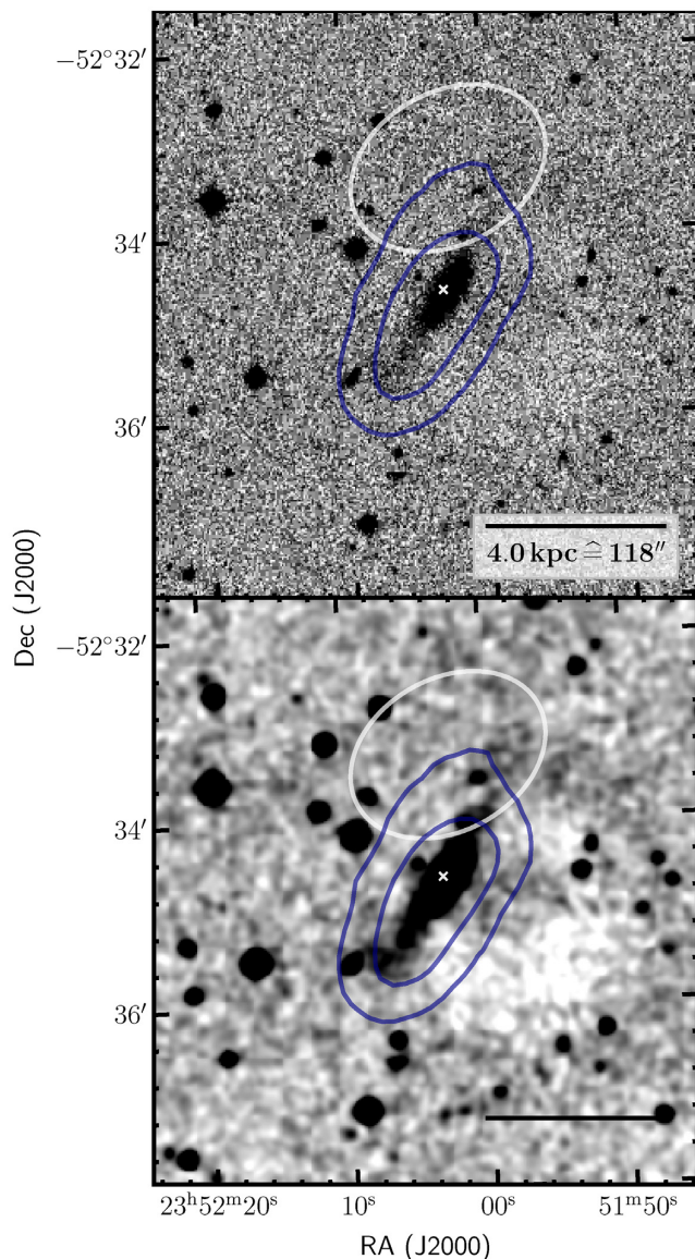
Figure 5. DSS (red, IIIa-F) images of ESO 149-G003. Blue contours denote the 1, 4- M_{\odot} \text{pc}^{-2} -levels of the observed total-intensity map shown in the left-hand panel of Figs 3 and A3. The white ellipse to the top in each image highlights the position of kinematically anomalous gas. The white cross represents the kinematical centre of the model. Top panel: full resolution. Bottom panel: image in top panel, convolved with a 2D-Gaussian of FWHM = 6 arcsec in each direction.
