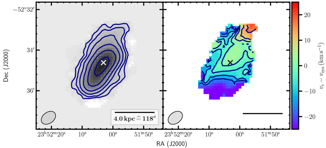
Figure A3. MeerKAT H I total-intensity map and moment-1 velocity field, as derived from the observed data cube shown in Figs 2, A2, and A1. The crosses represent the kinematical centre, the ellipse to the lower left-hand panel the synthesised beam ( HPWB ). Left-hand panel: Total-intensity map. Contours denote the 0.25, 0.5, 1, 2, 4, 8 M_{\odot} \text{pc}^{-2} -levels. Right-hand panel: velocity field. Contours are isovelocity contours. They denote the -15, -10, -5, 0, 5, 10, 15 \text{ km s}^{-1} -levels relative to the systemic velocity v_{\text{sys}} = 578 \text{ km s}^{-1} .
