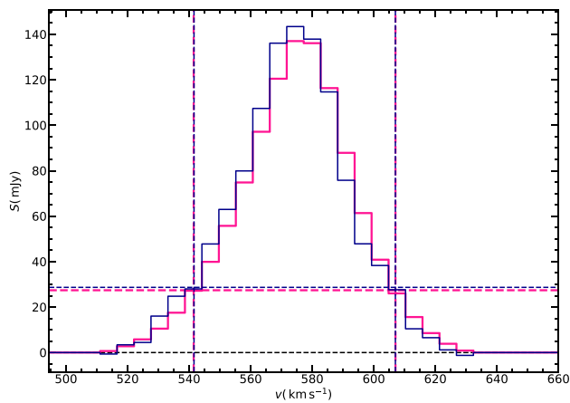
Figure A4. H I-spectrum of ESO 149-G003. Blue: observed. Pink: TiRiFiC model. The horizontal lines denote 20 per cent of the peak, the vertical lines the corresponding velocities.
