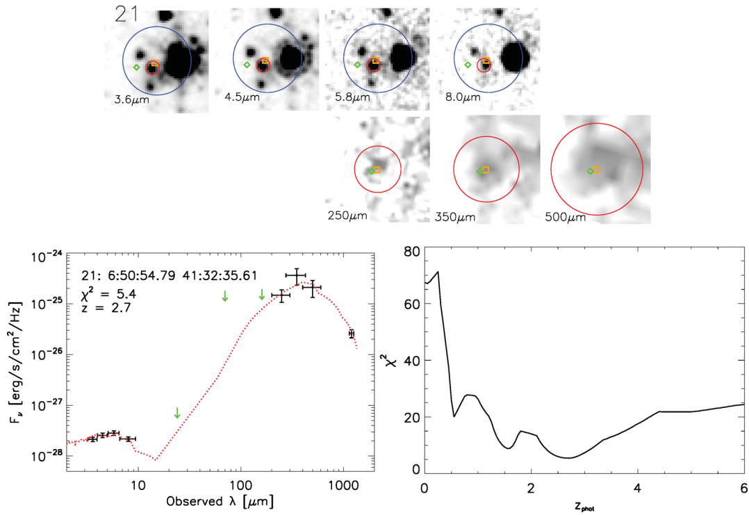
Figure A10. The stellar bump is clearly observed peaking between the IRAC2 and IRAC3 band. HYPERZ nicely fits this peak and puts this source at z_{\text{phot}} \sim 2.7 .
