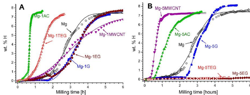
Fig. 1 – HRBM behaviour of Mg and Mg-C materials containing 1 (A) and 5 (B) wt.% of carbon additives: experimental data (symbols) and fitting results (lines).
