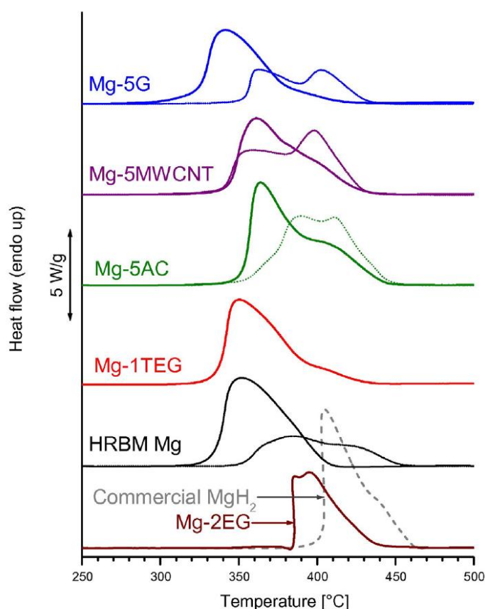
Fig. 6 – Typical DSC curves (heating rate 5\text{ }^{\circ}\text{C}/\text{min} ) for as-milled/as-delivered samples. The curves taken for air-exposed samples are shown as dotted lines.
