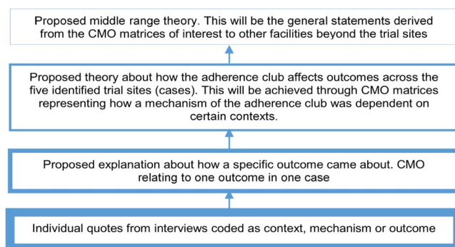
Figure 4 Analytical generalisation. 62
