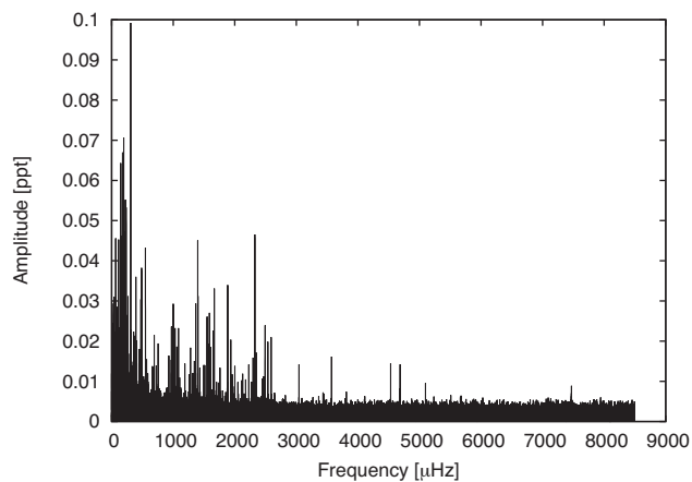
Figure 2. Amplitude spectrum of HW Vir after prewhitening of the orbital frequency comb, calculated up to the Nyquist frequency. A close-up of the region with frequencies up to 4800 \mu\text{Hz} is shown in Fig. 3.
