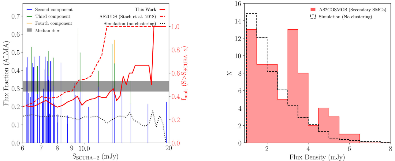
Figure 7. Left: The fraction of the integrated ALMA flux density that is contained in secondary components ( S_{870\ \mu\text{m}} > 1 mJy) in each AS2COSMOS map, as a function of the single-dish flux density of the targeted S2COSMOS source. Secondary AS2COSMOS SMGs contribute, on average, 30^{+3}_{-2} per cent (shaded region) of the integrated ALMA flux density with no significant dependence on SCUBA-2 flux density, in good agreement with results from AS2UDS for the same range in flux density ( 30 \pm 1 per cent; Stach et al. 2018). The fraction of AS2COSMOS maps that contain more than one SMG (solid line) shows a weak dependence on single-dish flux density, in broad agreement with the AS2UDS survey (dashed line; Stach et al. 2018). The level of multiplicity in the AS2COSMOS and AS2UDS samples is elevated relative to the expectations of an unclustered population (dotted line), which suggests that \sim 30 per cent of the AS2COSMOS ‘multiple’ maps contain physically associated SMGs. Right: The flux density distribution of the 76 secondary SMGs ( S_{870\ \mu\text{m}} > 1 mJy) that are detected within the primary beam of each AS2COSMOS map. For a comparison, we show the expected flux distribution of secondary components from our simulation of the A/S2COSMOS surveys, which assume an unclustered population of sub-millimetre sources. We find that the number density of secondary AS2COSMOS SMGs with flux densities of S_{870\ \mu\text{m}} < 3 mJy is broadly consistent with the results of our simulation, indicating that these faint SMGs are typically line-of-sight associations to the primary SMG in each ALMA map. However, we find a clear excess in the number density of AS2COSMOS secondaries brighter than S_{870\ \mu\text{m}} \gtrsim 3 mJy, relative to the simulation, and estimate that 62 \pm 7 per cent of these brighter components are physically associated with the primary SMG in their respective maps.
