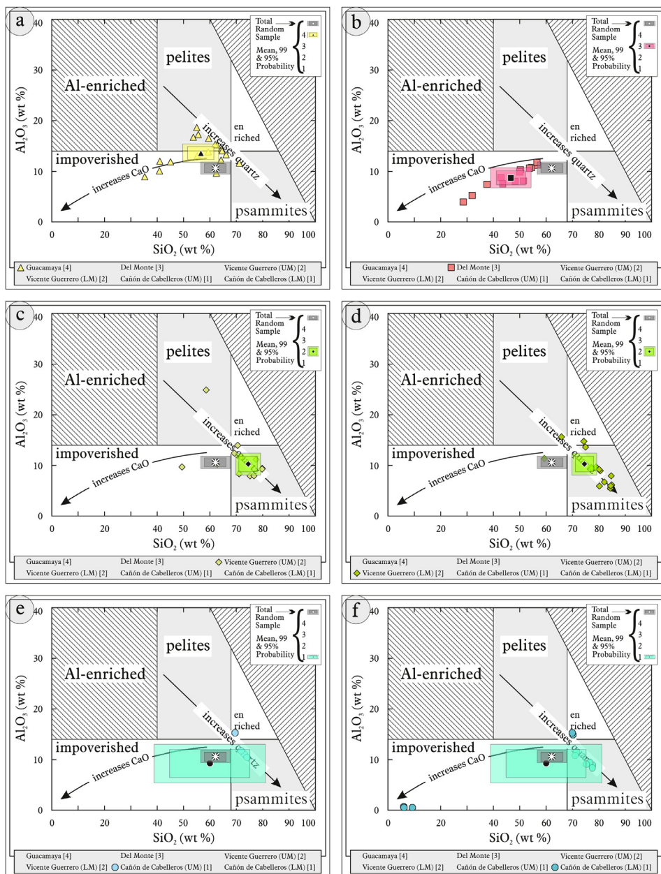
Fig. 16. Geochemical sediment classification of the Tamatán Group: SiO_2 - Al_2O_3 diagram after [10].
