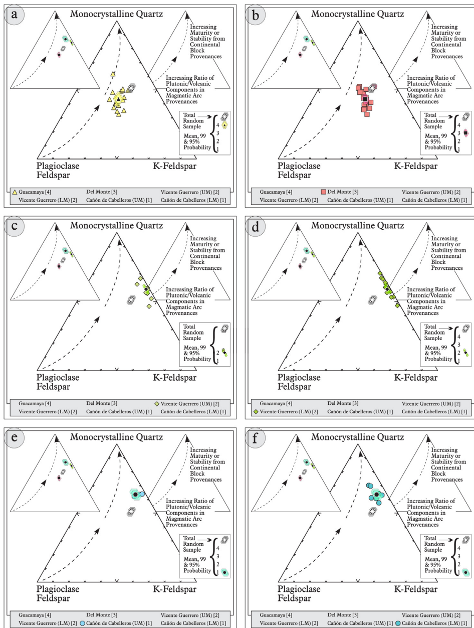
Fig. 13. Petrographic modal analysis of Tamatán Group sandstones: Qm–P–K after [6].
