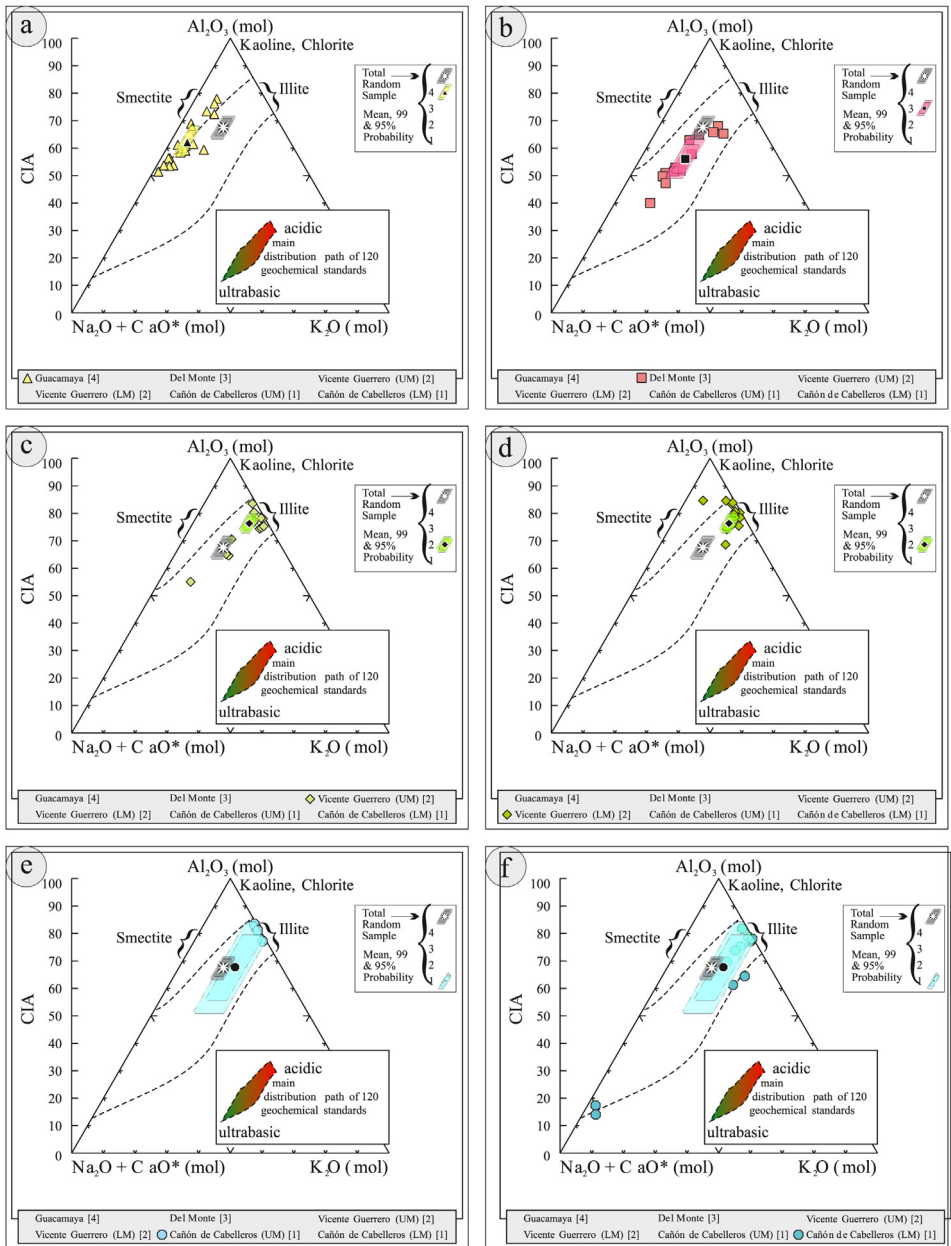
Fig. 18. Geochemical Index of Alteration of the sediments of the Tamatán Group: Na_2O+CaO-Al_2O_3-K_2O diagram after [12,13] modified by [10].
