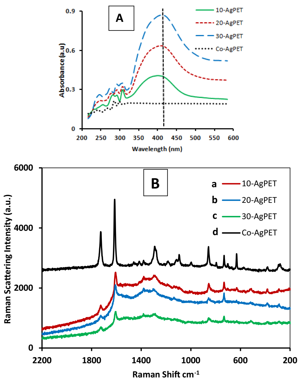
Fig. 5 A Ultraviolet–visible spectra of PET membranes coated at 90 °C and with 2 mL of 1% trisodium citrate for different immobilization times of 10 min (10-AgPET), 20 min (20-AgPET), 30 min (30-AgPET), and 0 min (Co-AgPET) and B Raman spectra of silver-coated track-etched PET membranes at reaction times (a) 10 min (10-AgPET), (b) 20 min (20-AgPET), and (c) 30 min (30-AgPET) and unmodified PET membrane (d) control (Co-AgPET) prepared at 90 °C using 2 mL of 1% trisodium citrate
