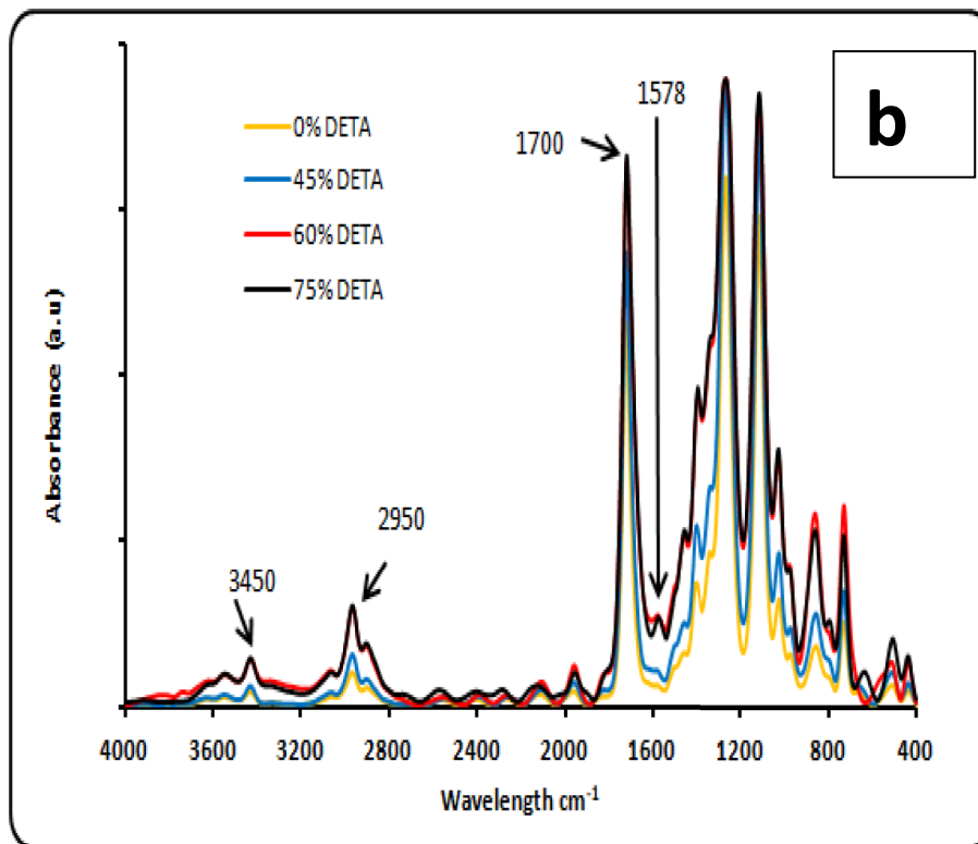
Fig. 1 a Proposed mechanism of modification of PET membrane with DETA and immobilisation of AgNPs on the modified surface and b FTIR spectra of unmodified PET membrane (CO-APET) and modi-
