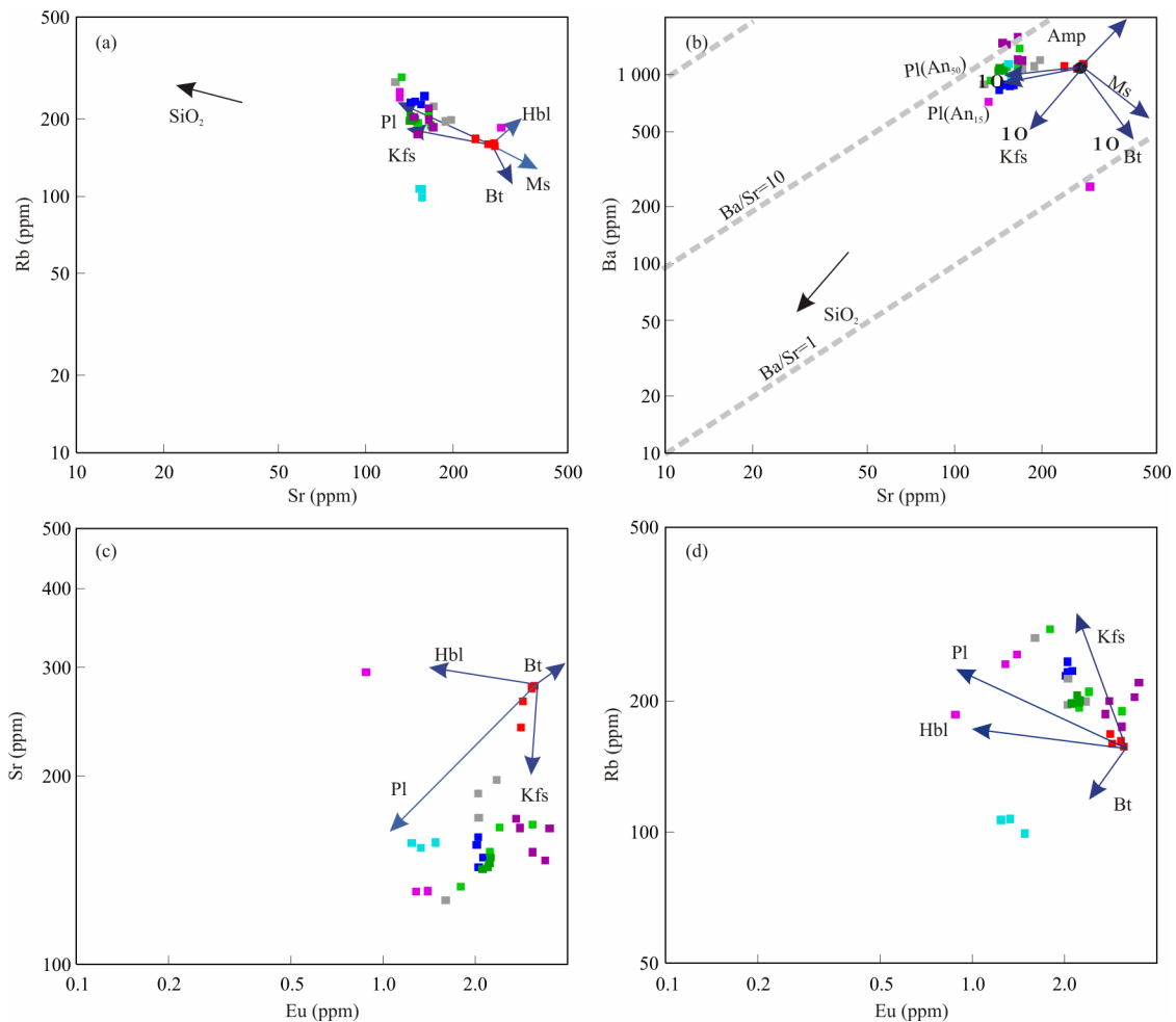
Figure 12. Binary plots testing the effects of fractional crystallisation of various minerals on the compositional variation within the Keimoos Suite granites. (a) Rb vs. Sr; (b) Ba vs. Sr; (c) Sr vs. Eu; (d) Rb vs. Eu.
