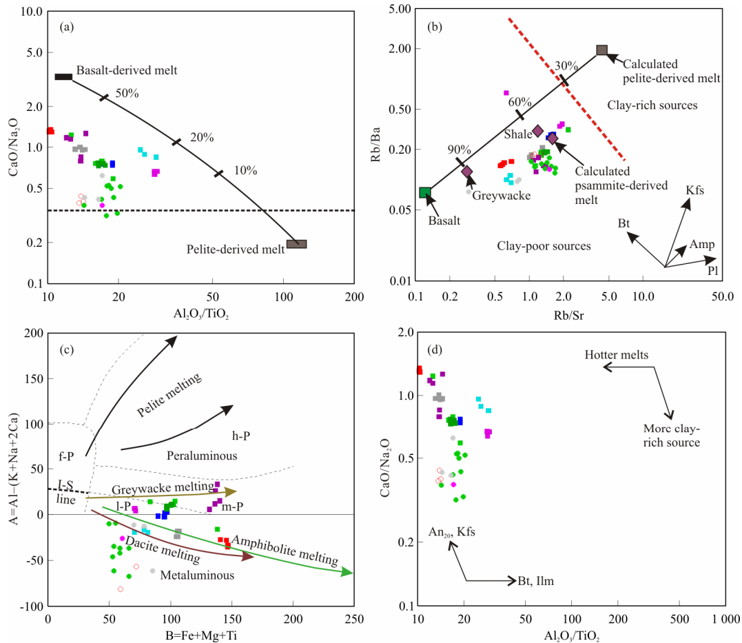
Figure 11. Test of source characteristics to the parental melts of the Koras Group volcanics and Keimoos Suite granitoids. (a) \text{CaO}/\text{Na}_2\text{O} vs. \text{Al}_2\text{O}_3/\text{TiO}_2 . (b) \text{Rb}/\text{Ba} vs. \text{Rb}/\text{Sr} . The mixing curve between basalt- and pelite-derived melts is from Patiño Douce and Harris (1998) and Sylvester (1998). (c) A-B diagram (after Villaseca et al., 1998). The arrows represent the compositions of progressive melt fractions produced by experimental melting of different crustal rocks (Villaseca et al., 1998 and references therein). Highly, moderately, low and highly felsic peraluminous granitoids, are indicated by h-P, m-P, l-P and f-P respectively. (d) \text{CaO}/\text{Na}_2\text{O} vs. \text{Al}_2\text{O}_3/\text{TiO}_2 plot. Vectors for fractional crystallization of oligoclase ( \text{An}_{20} ), K-feldspar (Kfs), biotite (Bt) and ilmenite (Ilm), and for illustrating compositional variations with increasing melting temperature and clay components in the source are from Sylvester (1998) and references therein.
