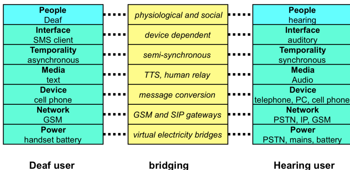
SIMBA v3 Softbridge stack
