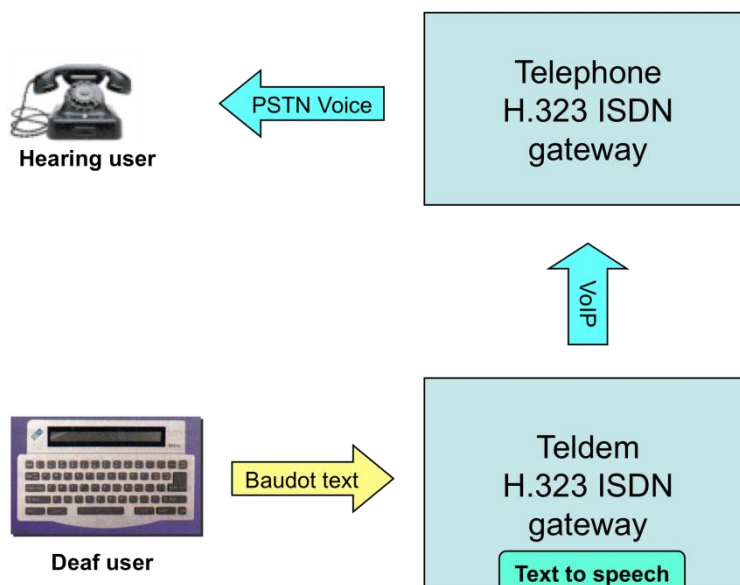
Telgo323 architecture
