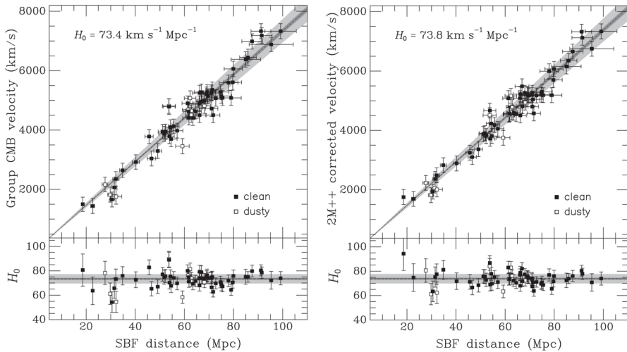
Fig. 40 Hubble diagrams and residuals from Blakeslee et al. (2021) based on Cepheid-calibrated WFC3/IR SBF distances tabulated by Jensen et al. (2021). The velocities are group-averaged values in the cosmic microwave background rest frame without correction for peculiar motions (left) and corrected using the 2 M++ flow model derived from the redshift-space density field analysis of Carrick et al. (2015). Solid symbols indicate “clean” galaxies, for which no dust or spiral structure is evident; open symbols are for galaxies with obvious dust and/or spiral structure. The best-fit Hubble constants are indicated, and the statistical and systematic error ranges are shown in dark and light gray, respectively. The reduced \chi^2 improves from 0.97 for the fit on the left to 0.89 for the fit using the flow-model, but the value of H_0 depends on the overall velocity scale factor, and the study adopted the model-independent version for this. H_0 would increase by 0.3% for the TRGB-based SBF calibration. Image reproduced with permission from Blakeslee et al. (2021), copyright by the authors
