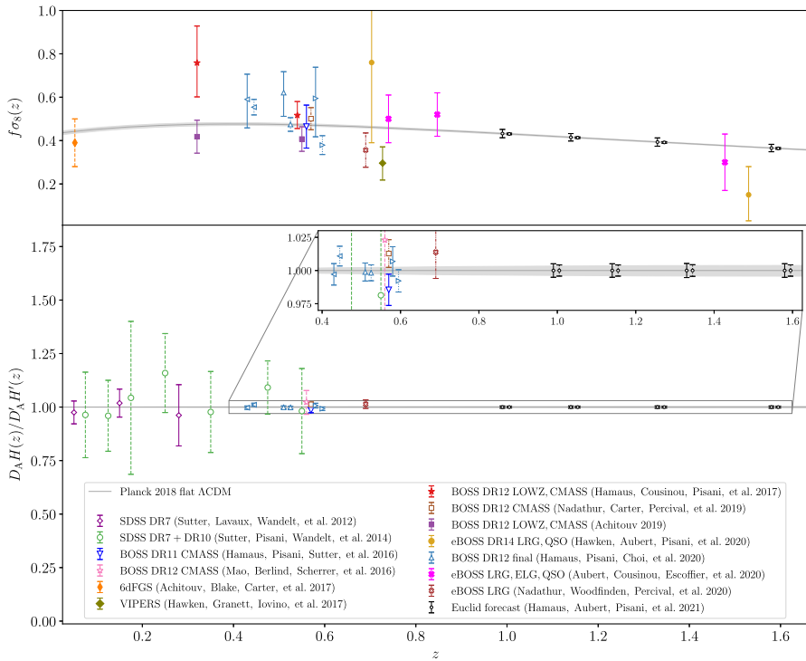
Fig. 31 Comparison of constraints on growth via f_{\sigma_8} and geometry via D_A H (68% confidence intervals) obtained from cosmic voids in the literature, references are ordered chronologically in the figure legend. Gray lines with shaded error bands show the Planck Collaboration et al. (2020) baseline result as a reference, with corresponding values of D_A^* H' . Filled markers indicate growth rate measurements without consideration of the AP effect, while open markers include the AP test. The different line styles of error bars indicate various degrees of model assumptions made: model-independent (solid), calibrated on simulations (dashed), calibrated on mocks (dotted), calibrated on simulations and mocks (dash-dotted)
