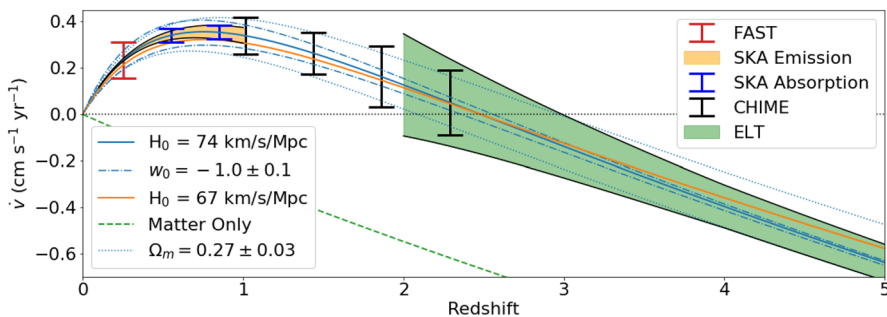
Fig. 47 Forecast acceleration measurements versus redshift for the SKA using H \alpha 21-cm emission from galaxies (Kloekner et al. 2015), CHIME using H \alpha 21-cm absorption (Yu et al. 2014), H \alpha 21-cm absorption using FAST and the SKA estimated from projected detections (see text), and an ELT program that monitors the Ly \alpha forest (Liske et al. 2008). The cosmological tracks follow Fig. 46. The shaded loci and error bars indicate 1\sigma uncertainties
