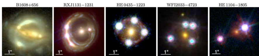
Fig. 20 Four quadruply lensed quasar systems and one doubly lensed quasar system from the H0LiCOW sample. The lens name is indicated above each panel. The color images are composed using 2 (for B1608+656) or 3 (for other lenses) HST imaging bands in the optical and near-infrared. North is up and east is left. Image reproduced with permission from Suyu et al. (2017), copyright by the authors
