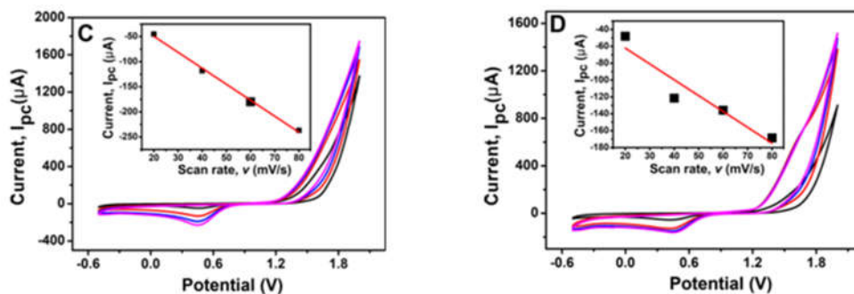
Figure 3. Cyclic voltammograms of HL (C) and ZnL_2 (D). Inset: calibration curve of I_{pc} versus v at scan rates 20, 40, 60, and 80 \text{ mV s}^{-1} in 0.01 M PBS, pH 7.4.
