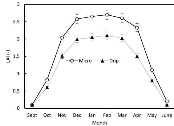
Fig. 2. Seasonal changes in the tree leaf area index (LAI) of the Royal gala trees under different irrigation systems.
